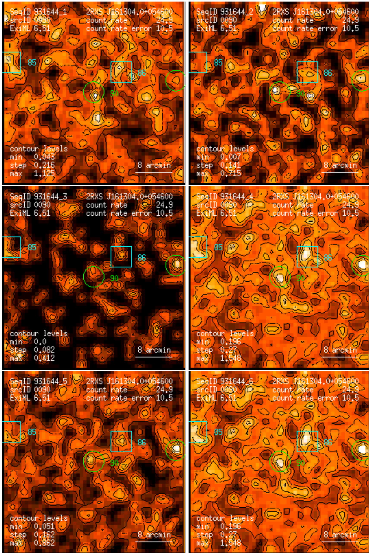
Figure 90: RASS 931644: detection 0090: band rate images, Gaussian filter: (1) PSPC channels 11 – 41, (2) 52 – 90, (3) 91 – 201, (4) 11 – 235, (5) 52 – 201, (6) 11 – 201. Broad band rates in counts/ks. Band rate contour levels in counts/ks/arcmin 2 .
