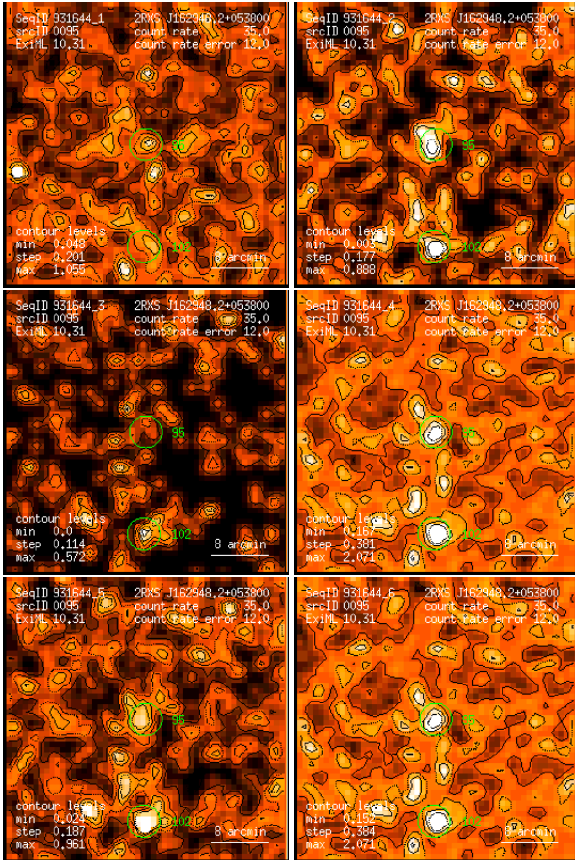
Figure 95: RASS 931644: detection 0095: band rate images, Gaussian filter: (1) PSPC channels 11 – 41, (2) 52 – 90, (3) 91 – 201, (4) 11 – 235, (5) 52 – 201, (6) 11 – 201. Broad band rates in counts/ks. Band rate contour levels in counts/ks/arcmin 2 .
