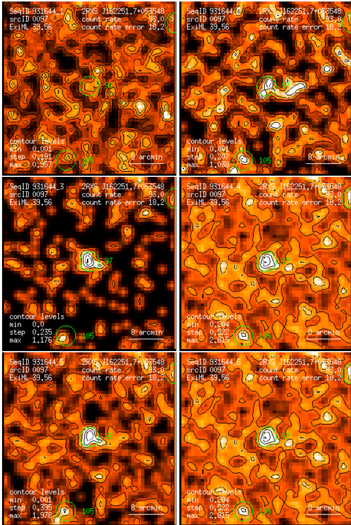
Figure 97: RASS 931644: detection 0097: band rate images, Gaussian filter: (1) PSPC channels 11 – 41, (2) 52 – 90, (3) 91 – 201, (4) 11 – 235, (5) 52 – 201, (6) 11 – 201. Broad band rates in counts/ks. Band rate contour levels in counts/ks/arcmin 2 .
