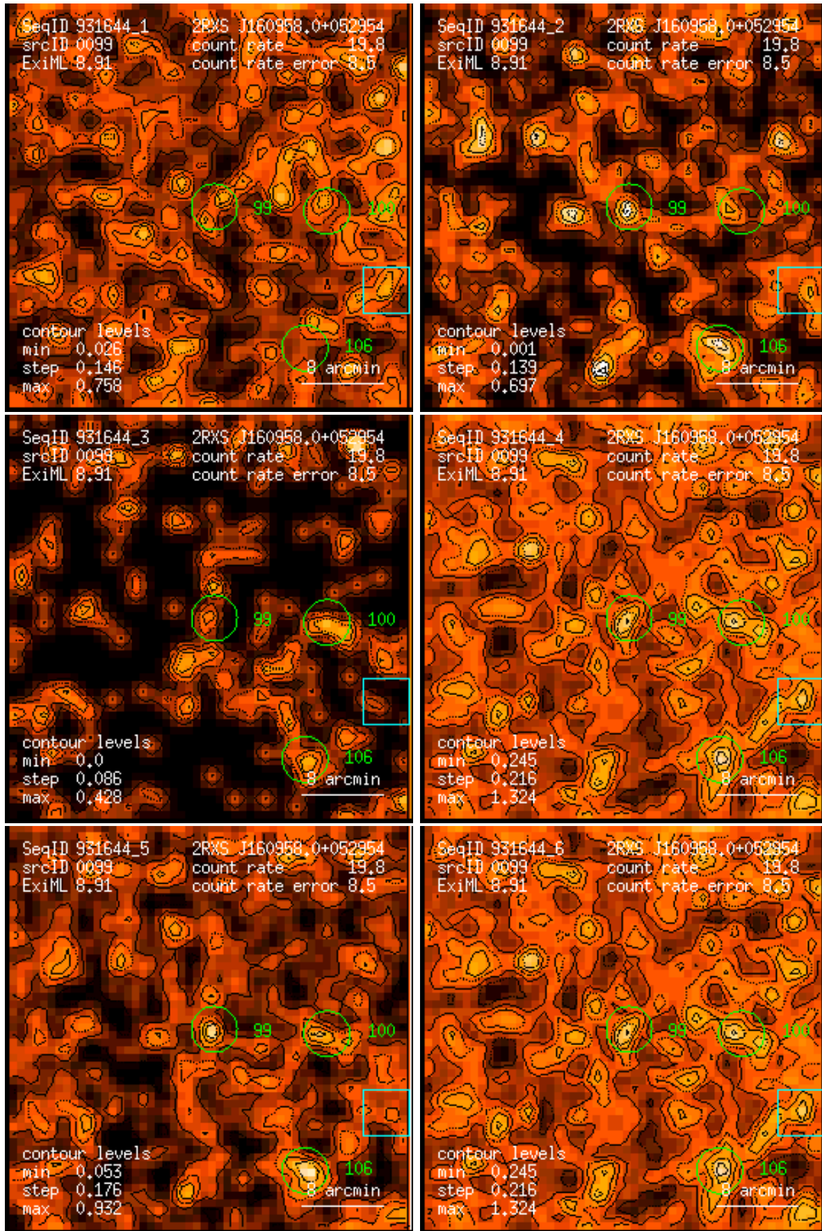
Figure 99: RASS 931644: detection 0099: band rate images, Gaussian filter: (1) PSPC channels 11 – 41, (2) 52 – 90, (3) 91 – 201, (4) 11 – 235, (5) 52 – 201, (6) 11 – 201. Broad band rates in counts/ks. Band rate contour levels in counts/ks/arcmin 2 .
