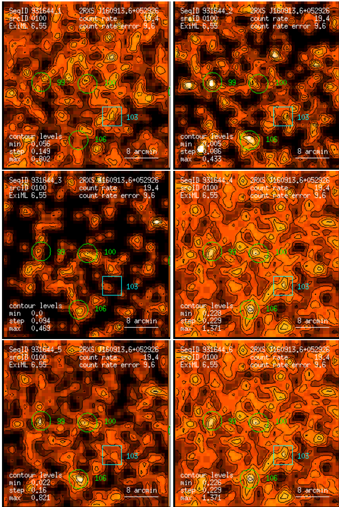
Figure 100: RASS 931644: detection 0100: band rate images, Gaussian filter: (1) PSPC channels 11 – 41, (2) 52 – 90, (3) 91 – 201, (4) 11 – 235, (5) 52 – 201, (6) 11 – 201. Broad band rates in counts/ks. Band rate contour levels in counts/ks/arcmin 2 .
