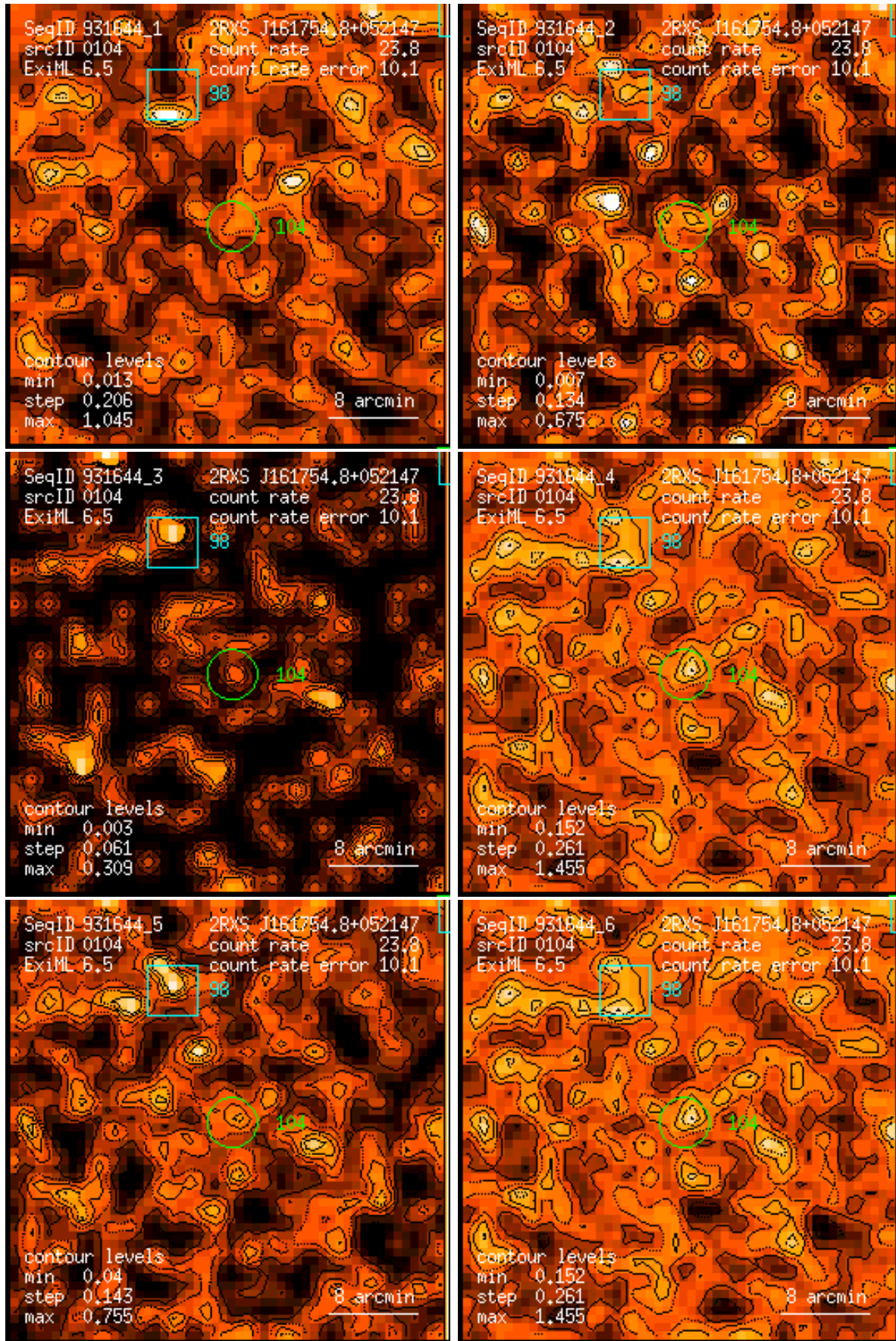
Figure 104: RASS 931644: detection 0104: band rate images, Gaussian filter: (1) PSPC channels 11 – 41, (2) 52 – 90, (3) 91 – 201, (4) 11 – 235, (5) 52 – 201, (6) 11 – 201. Broad band rates in counts/ks. Band rate contour levels in counts/ks/arcmin 2 .
