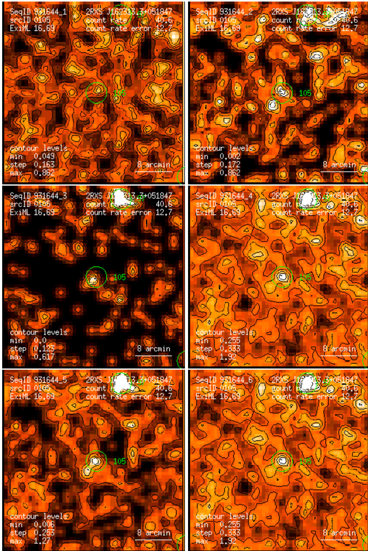
Figure 105: RASS 931644: detection 0105: band rate images, Gaussian filter: (1) PSPC channels 11 – 41, (2) 52 – 90, (3) 91 – 201, (4) 11 – 235, (5) 52 – 201, (6) 11 – 201. Broad band rates in counts/ks. Band rate contour levels in counts/ks/arcmin 2 .
