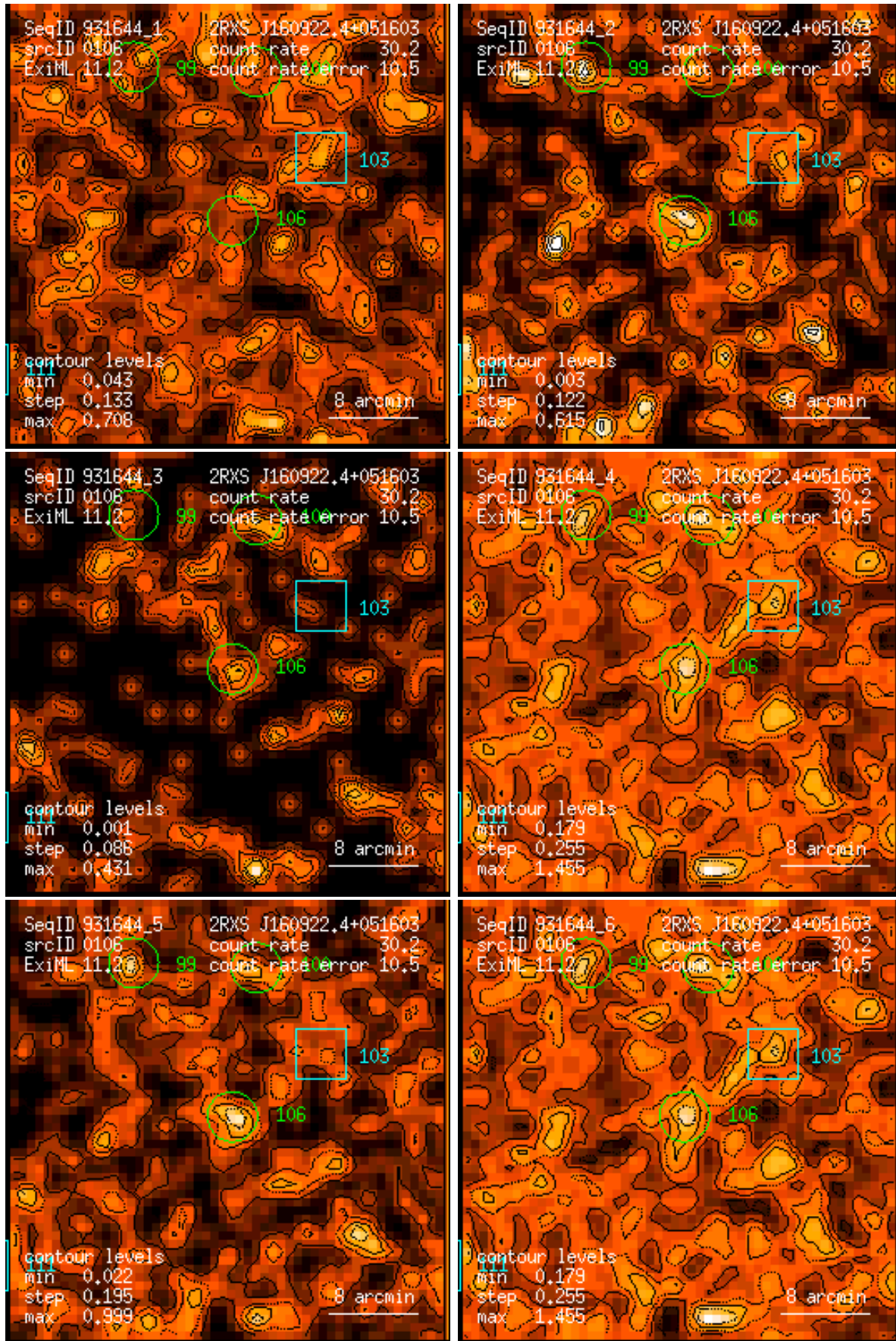
Figure 106: RASS 931644: detection 0106: band rate images, Gaussian filter: (1) PSPC channels 11 – 41, (2) 52 – 90, (3) 91 – 201, (4) 11 – 235, (5) 52 – 201, (6) 11 – 201. Broad band rates in counts/ks. Band rate contour levels in counts/ks/arcmin 2 .
