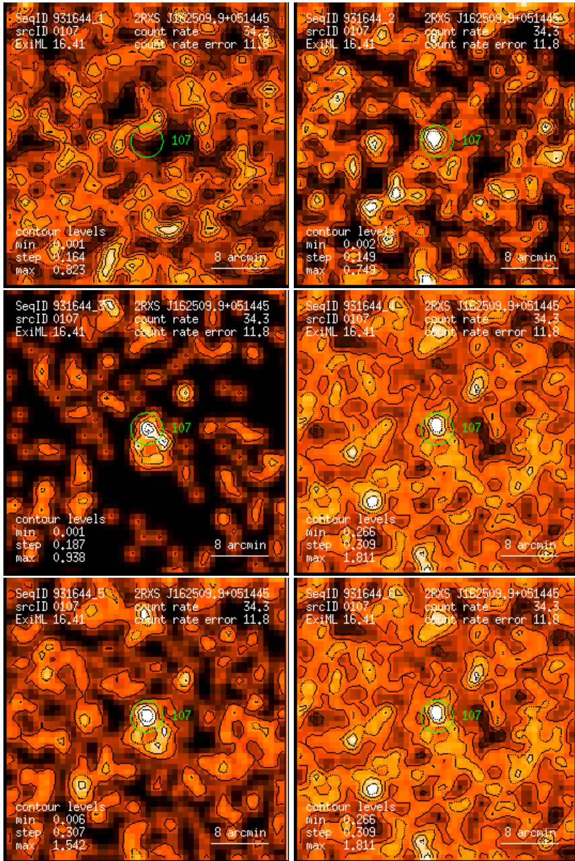
Figure 107: RASS 931644: detection 0107: band rate images, Gaussian filter: (1) PSPC channels 11 – 41, (2) 52 – 90, (3) 91 – 201, (4) 11 – 235, (5) 52 – 201, (6) 11 – 201. Broad band rates in counts/ks. Band rate contour levels in counts/ks/arcmin 2 .
