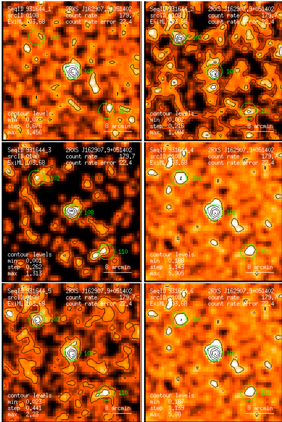
Figure 108: RASS 931644: detection 0108: band rate images, Gaussian filter: (1) PSPC channels 11 – 41, (2) 52 – 90, (3) 91 – 201, (4) 11 – 235, (5) 52 – 201, (6) 11 – 201. Broad band rates in counts/ks. Band rate contour levels in counts/ks/arcmin 2 .
