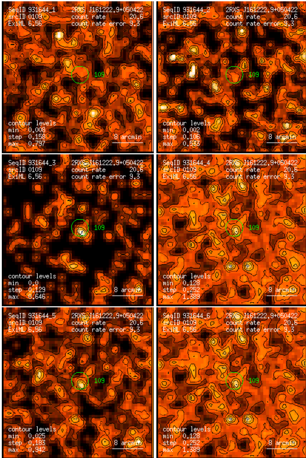
Figure 109: RASS 931644: detection 0109: band rate images, Gaussian filter: (1) PSPC channels 11 – 41, (2) 52 – 90, (3) 91 – 201, (4) 11 – 235, (5) 52 – 201, (6) 11 – 201. Broad band rates in counts/ks. Band rate contour levels in counts/ks/arcmin 2 .
