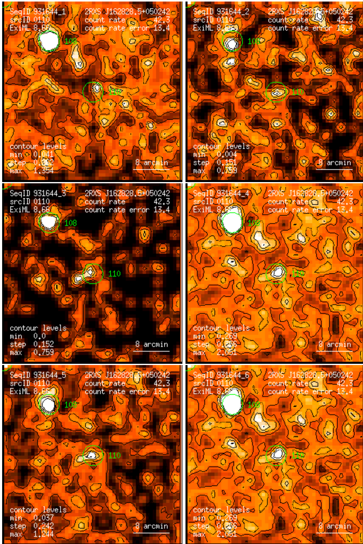
Figure 110: RASS 931644: detection 0110: band rate images, Gaussian filter: (1) PSPC channels 11 – 41, (2) 52 – 90, (3) 91 – 201, (4) 11 – 235, (5) 52 – 201, (6) 11 – 201. Broad band rates in counts/ks. Band rate contour levels in counts/ks/arcmin 2 .
