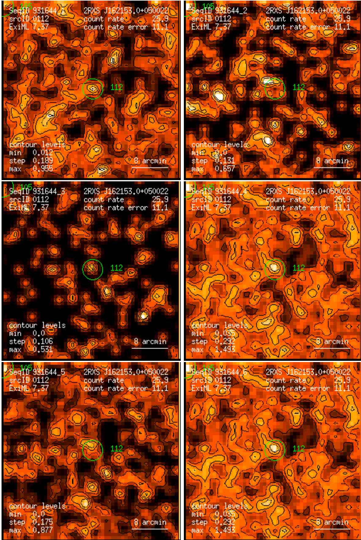
Figure 112: RASS 931644: detection 0112: band rate images, Gaussian filter: (1) PSPC channels 11 – 41, (2) 52 – 90, (3) 91 – 201, (4) 11 – 235, (5) 52 – 201, (6) 11 – 201. Broad band rates in counts/ks. Band rate contour levels in counts/ks/arcmin 2 .
