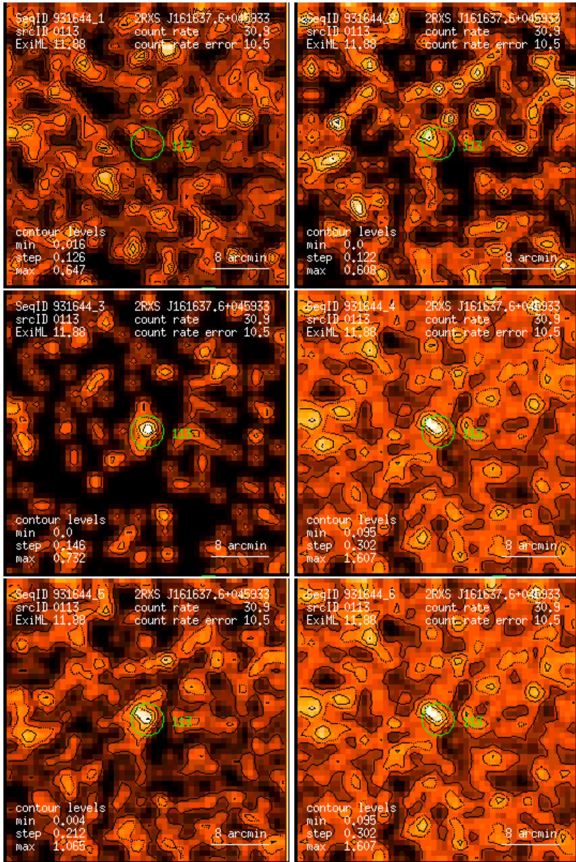
Figure 113: RASS 931644: detection 0113: band rate images, Gaussian filter: (1) PSPC channels 11 – 41, (2) 52 – 90, (3) 91 – 201, (4) 11 – 235, (5) 52 – 201, (6) 11 – 201. Broad band rates in counts/ks. Band rate contour levels in counts/ks/arcmin 2 .
