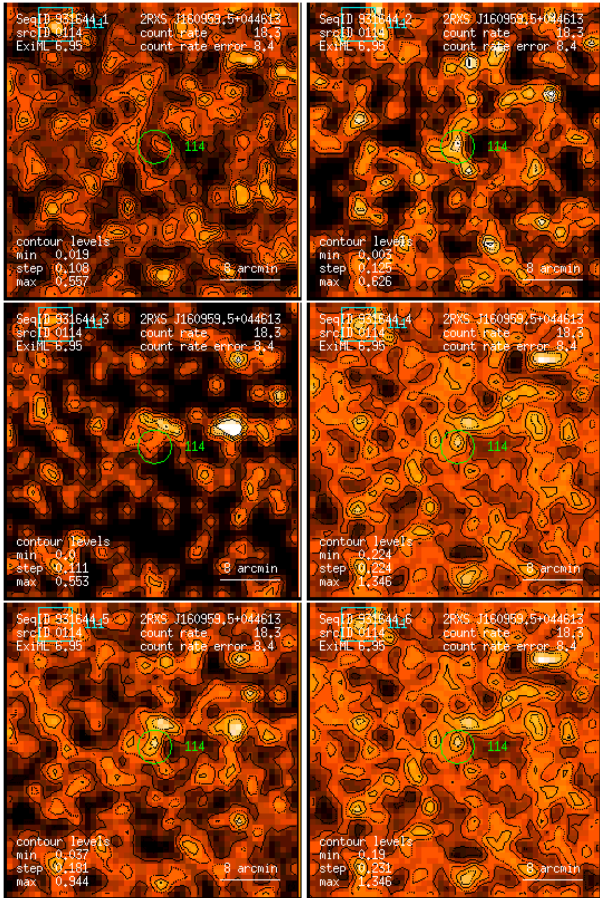
Figure 114: RASS 931644: detection 0114: band rate images, Gaussian filter: (1) PSPC channels 11 – 41, (2) 52 – 90, (3) 91 – 201, (4) 11 – 235, (5) 52 – 201, (6) 11 – 201. Broad band rates in counts/ks. Band rate contour levels in counts/ks/arcmin 2 .
