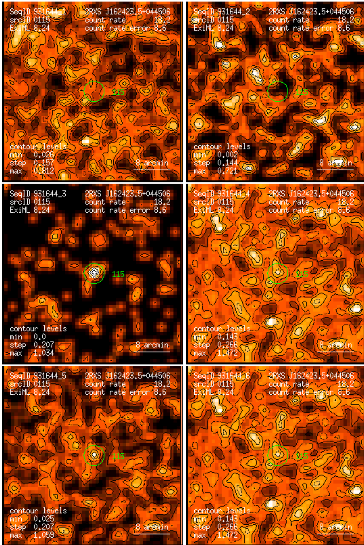
Figure 115: RASS 931644: detection 0115: band rate images, Gaussian filter: (1) PSPC channels 11 – 41, (2) 52 – 90, (3) 91 – 201, (4) 11 – 235, (5) 52 – 201, (6) 11 – 201. Broad band rates in counts/ks. Band rate contour levels in counts/ks/arcmin 2 .
