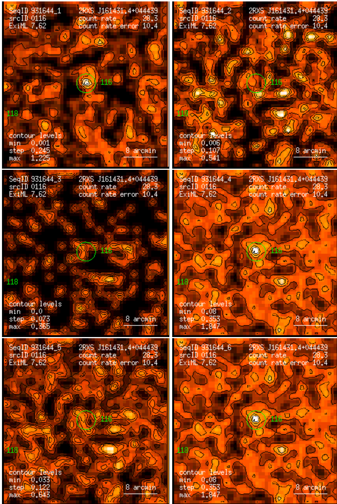
Figure 116: RASS 931644: detection 0116: band rate images, Gaussian filter: (1) PSPC channels 11 – 41, (2) 52 – 90, (3) 91 – 201, (4) 11 – 235, (5) 52 – 201, (6) 11 – 201. Broad band rates in counts/ks. Band rate contour levels in counts/ks/arcmin 2 .
