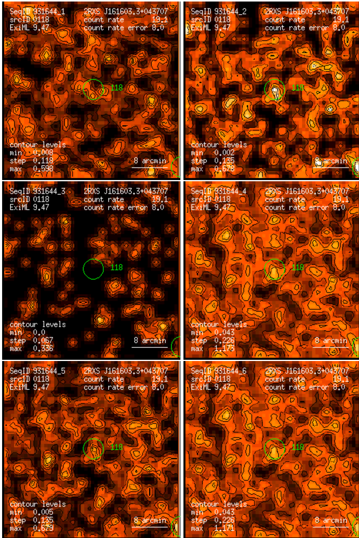
Figure 118: RASS 931644: detection 0118: band rate images, Gaussian filter: (1) PSPC channels 11 – 41, (2) 52 – 90, (3) 91 – 201, (4) 11 – 235, (5) 52 – 201, (6) 11 – 201. Broad band rates in counts/ks. Band rate contour levels in counts/ks/arcmin 2 .
