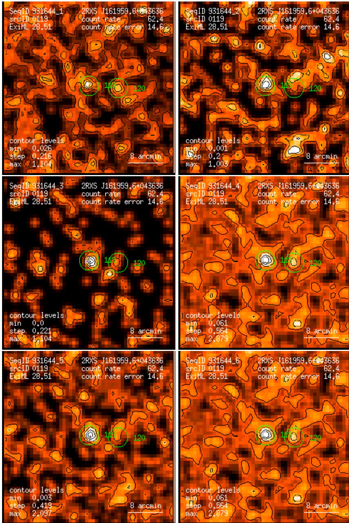
Figure 119: RASS 931644: detection 0119: band rate images, Gaussian filter: (1) PSPC channels 11 – 41, (2) 52 – 90, (3) 91 – 201, (4) 11 – 235, (5) 52 – 201, (6) 11 – 201. Broad band rates in counts/ks. Band rate contour levels in counts/ks/arcmin 2 .
