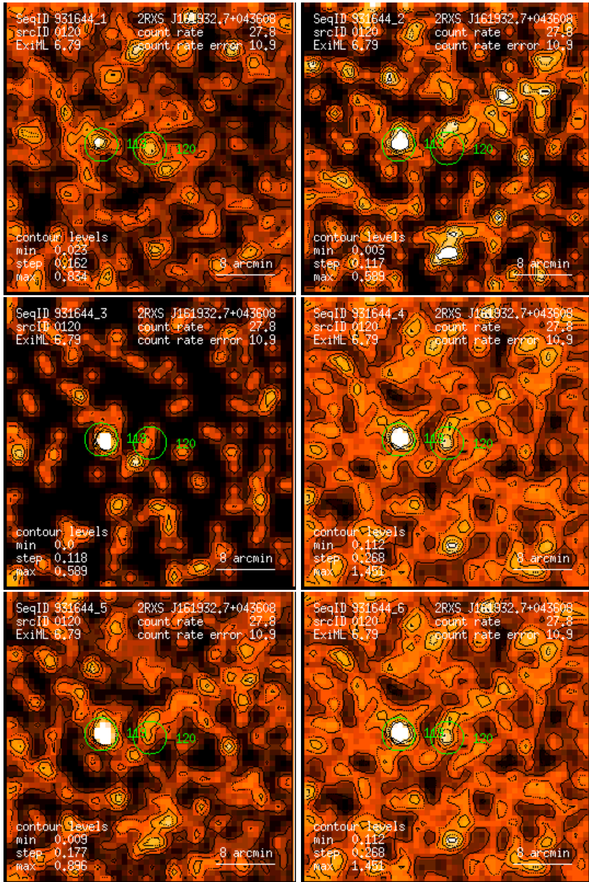
Figure 120: RASS 931644: detection 0120: band rate images, Gaussian filter: (1) PSPC channels 11 – 41, (2) 52 – 90, (3) 91 – 201, (4) 11 – 235, (5) 52 – 201, (6) 11 – 201. Broad band rates in counts/ks. Band rate contour levels in counts/ks/arcmin 2 .
