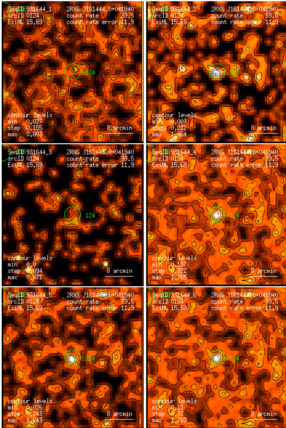
Figure 124: RASS 931644: detection 0124: band rate images, Gaussian filter: (1) PSPC channels 11 – 41, (2) 52 – 90, (3) 91 – 201, (4) 11 – 235, (5) 52 – 201, (6) 11 – 201. Broad band rates in counts/ks. Band rate contour levels in counts/ks/arcmin 2 .
