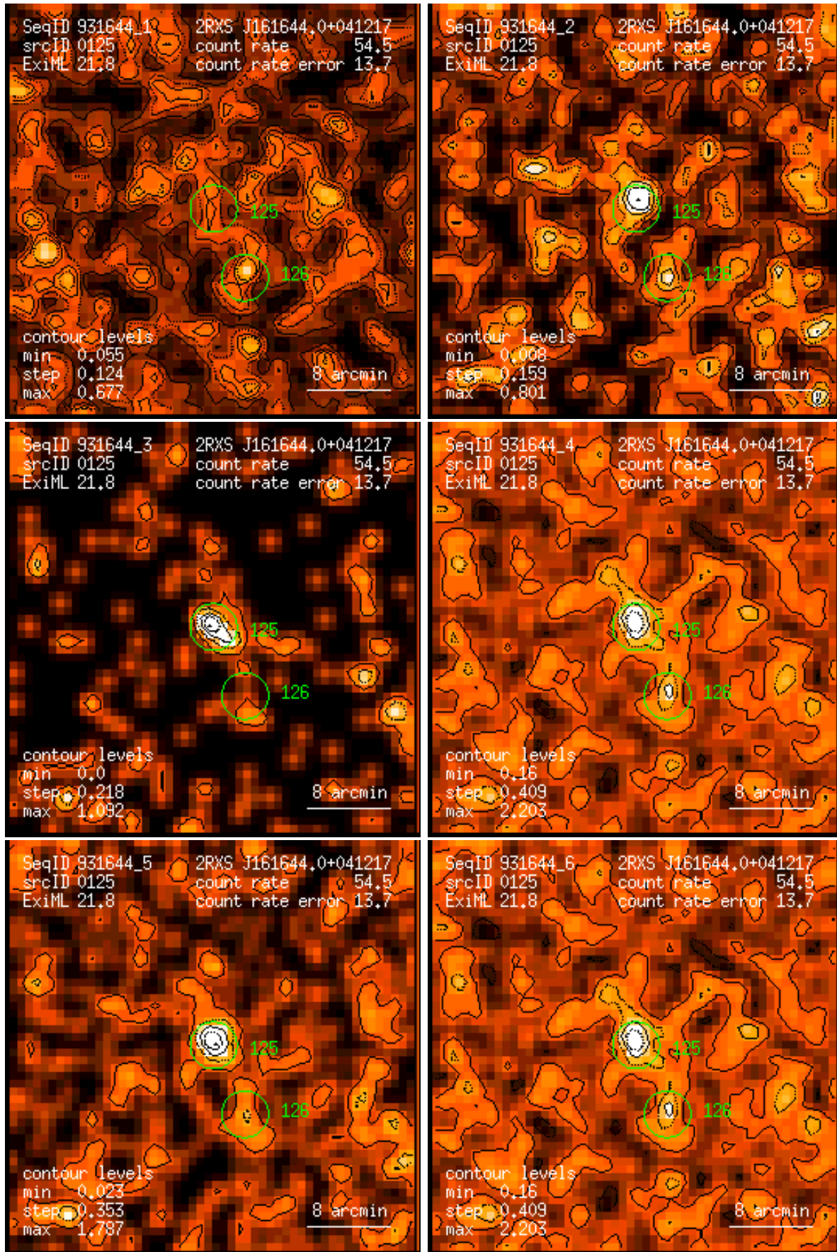
Figure 125: RASS 931644: detection 0125: band rate images, Gaussian filter: (1) PSPC channels 11 – 41, (2) 52 – 90, (3) 91 – 201, (4) 11 – 235, (5) 52 – 201, (6) 11 – 201. Broad band rates in counts/ks. Band rate contour levels in counts/ks/arcmin 2 .
