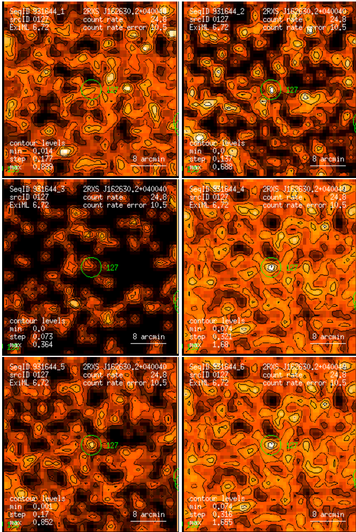
Figure 127: RASS 931644: detection 0127: band rate images, Gaussian filter: (1) PSPC channels 11 – 41, (2) 52 – 90, (3) 91 – 201, (4) 11 – 235, (5) 52 – 201, (6) 11 – 201. Broad band rates in counts/ks. Band rate contour levels in counts/ks/arcmin 2 .
