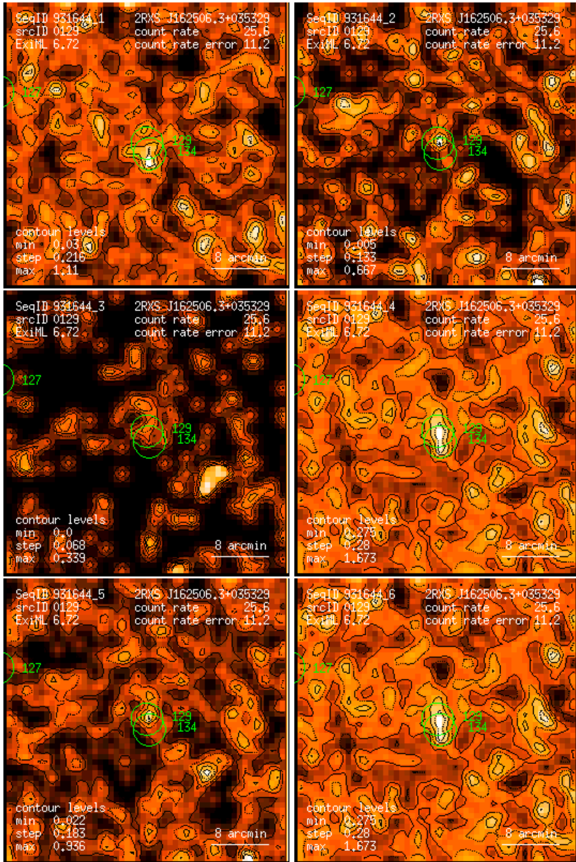
Figure 129: RASS 931644: detection 0129: band rate images, Gaussian filter: (1) PSPC channels 11 – 41, (2) 52 – 90, (3) 91 – 201, (4) 11 – 235, (5) 52 – 201, (6) 11 – 201. Broad band rates in counts/ks. Band rate contour levels in counts/ks/arcmin 2 .
