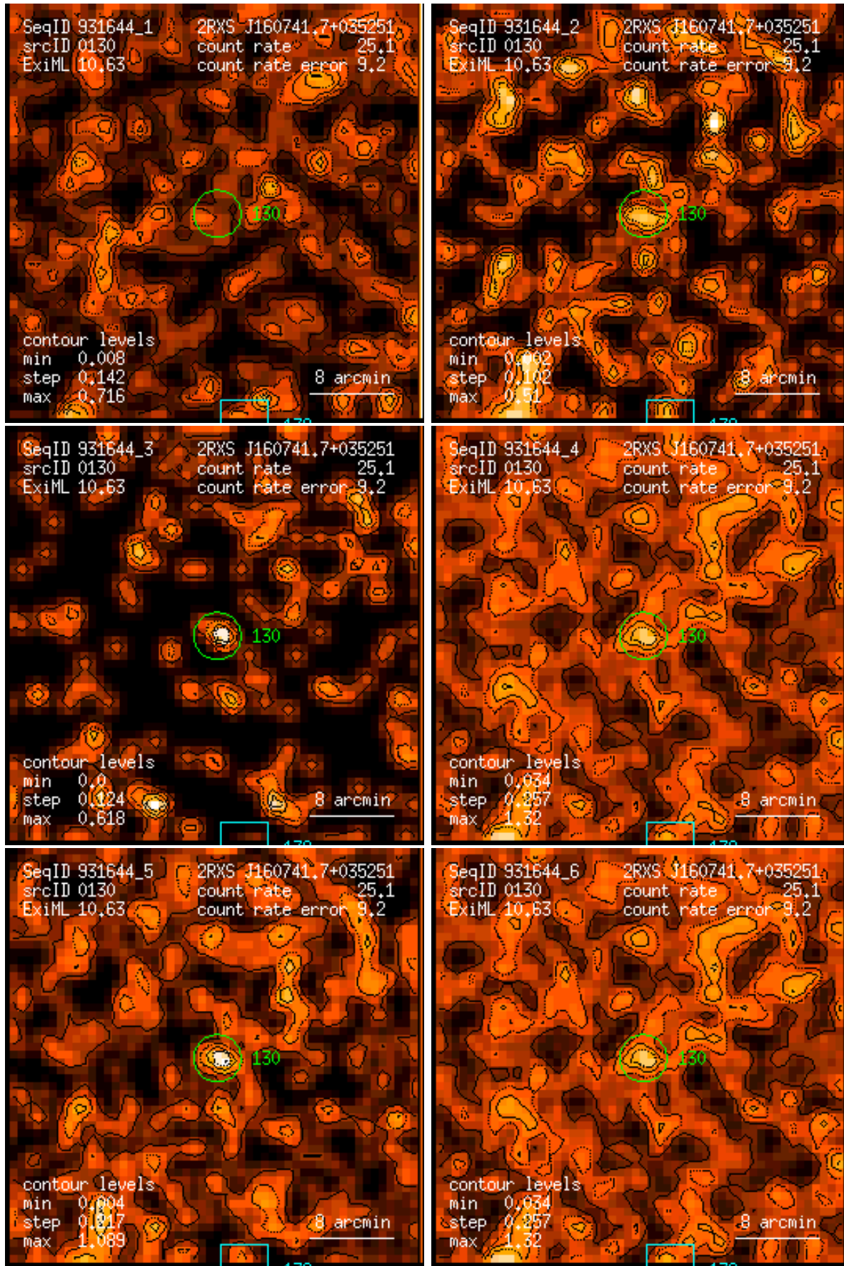
Figure 130: RASS 931644: detection 0130: band rate images, Gaussian filter: (1) PSPC channels 11 – 41, (2) 52 – 90, (3) 91 – 201, (4) 11 – 235, (5) 52 – 201, (6) 11 – 201. Broad band rates in counts/ks. Band rate contour levels in counts/ks/arcmin 2 .
