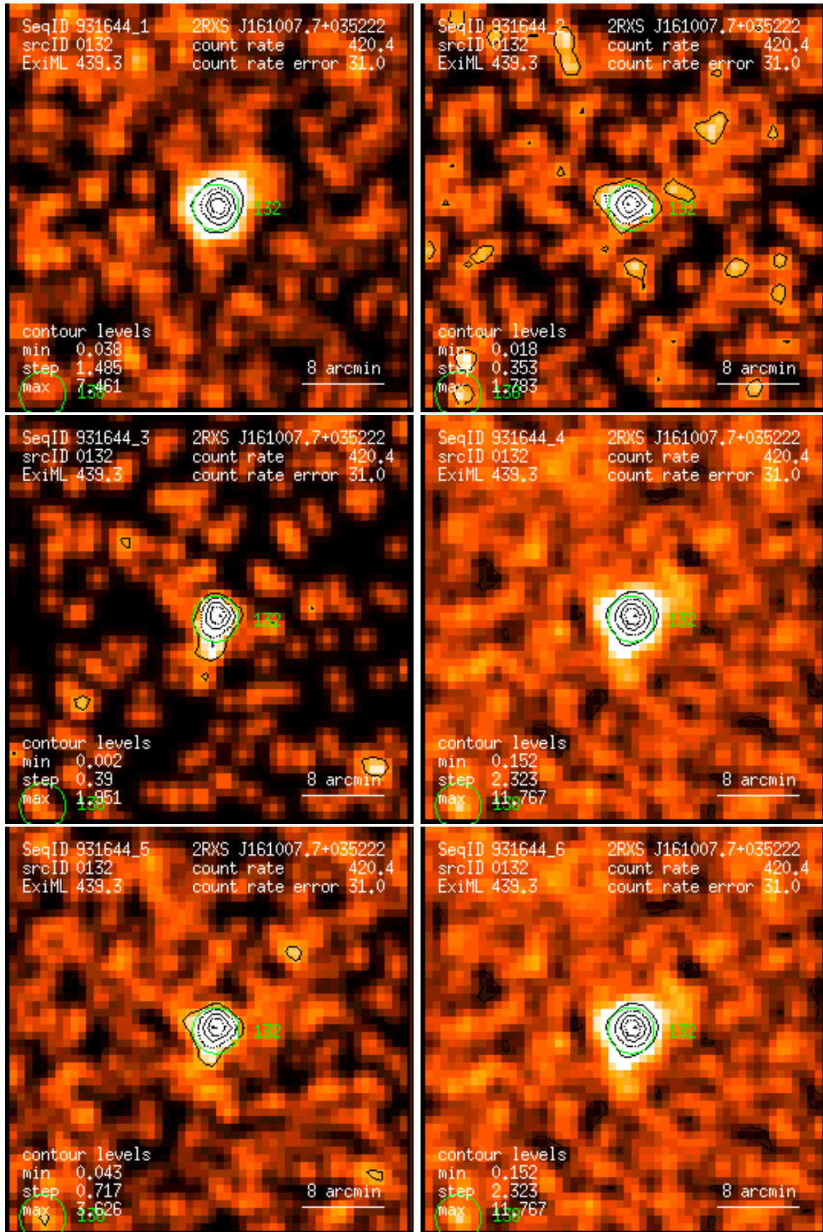
Figure 132: RASS 931644: detection 0132: band rate images, Gaussian filter: (1) PSPC channels 11 – 41, (2) 52 – 90, (3) 91 – 201, (4) 11 – 235, (5) 52 – 201, (6) 11 – 201. Broad band rates in counts/ks. Band rate contour levels in counts/ks/arcmin 2 .
