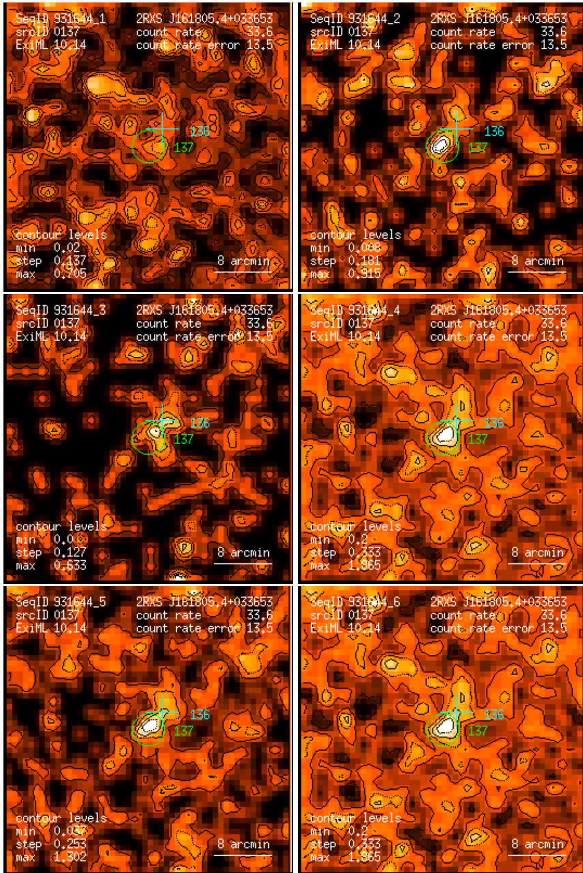
Figure 137: RASS 931644: detection 0137: band rate images, Gaussian filter: (1) PSPC channels 11 – 41, (2) 52 – 90, (3) 91 – 201, (4) 11 – 235, (5) 52 – 201, (6) 11 – 201. Broad band rates in counts/ks. Band rate contour levels in counts/ks/arcmin 2 .
