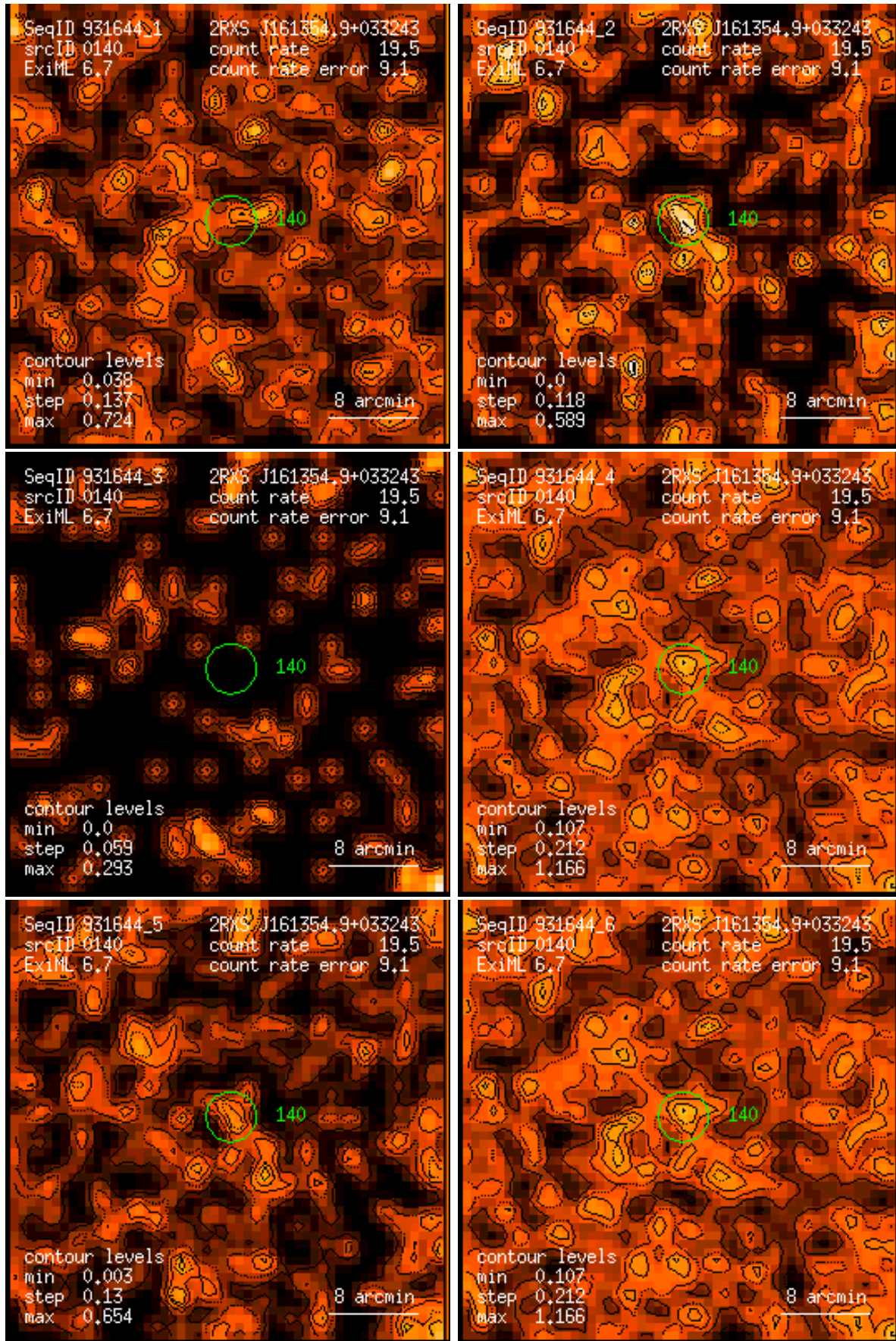
Figure 140: RASS 931644: detection 0140: band rate images, Gaussian filter: (1) PSPC channels 11 – 41, (2) 52 – 90, (3) 91 – 201, (4) 11 – 235, (5) 52 – 201, (6) 11 – 201. Broad band rates in counts/ks. Band rate contour levels in counts/ks/arcmin 2 .
