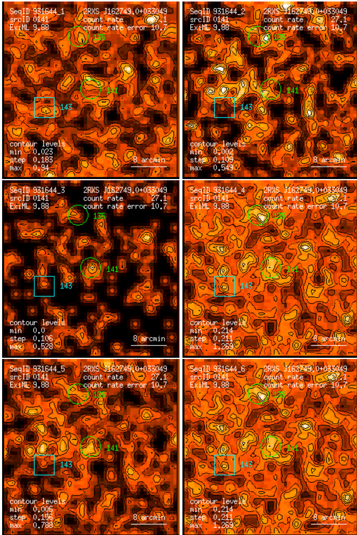
Figure 141: RASS 931644: detection 0141: band rate images, Gaussian filter: (1) PSPC channels 11 – 41, (2) 52 – 90, (3) 91 – 201, (4) 11 – 235, (5) 52 – 201, (6) 11 – 201. Broad band rates in counts/ks. Band rate contour levels in counts/ks/arcmin 2 .
