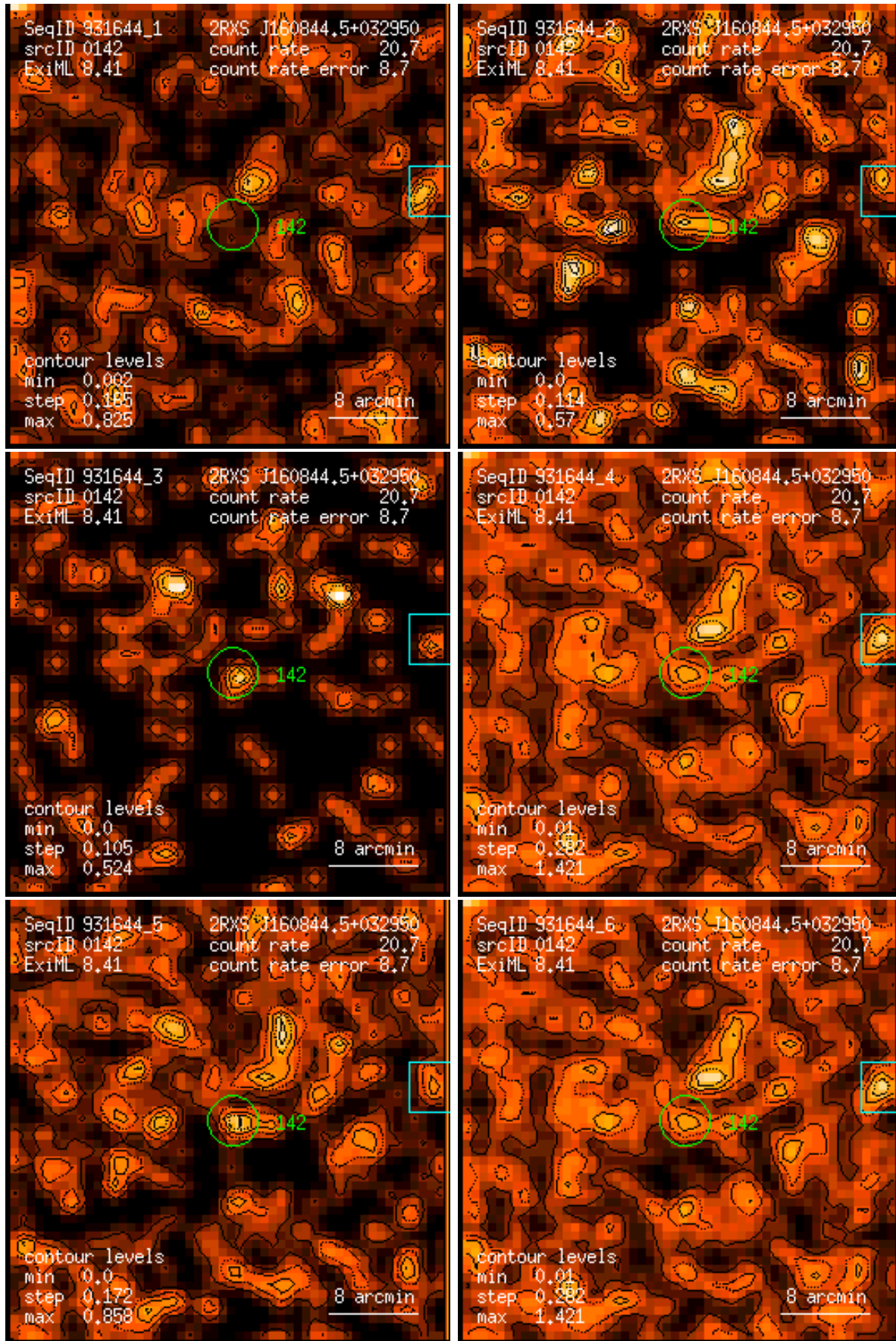
Figure 142: RASS 931644: detection 0142: band rate images, Gaussian filter: (1) PSPC channels 11 – 41, (2) 52 – 90, (3) 91 – 201, (4) 11 – 235, (5) 52 – 201, (6) 11 – 201. Broad band rates in counts/ks. Band rate contour levels in counts/ks/arcmin 2 .
