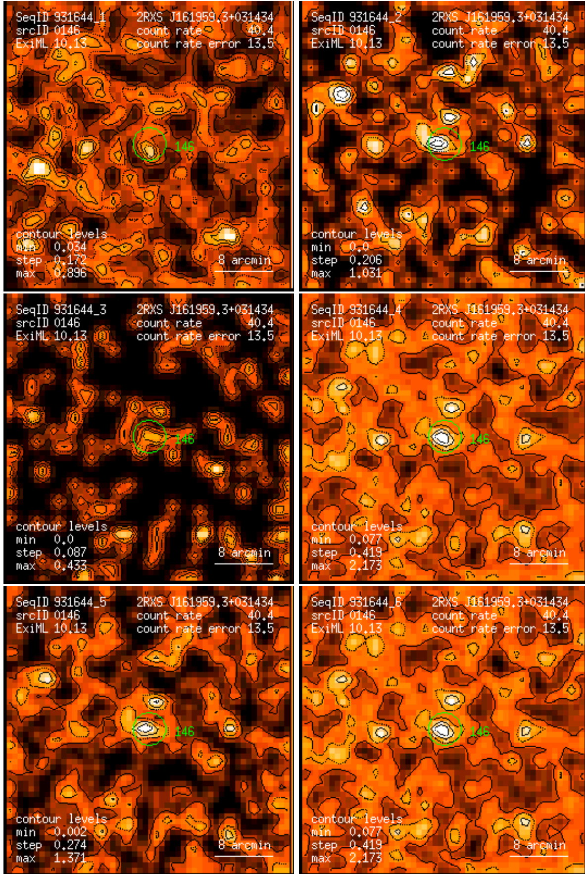
Figure 146: RASS 931644: detection 0146: band rate images, Gaussian filter: (1) PSPC channels 11 – 41, (2) 52 – 90, (3) 91 – 201, (4) 11 – 235, (5) 52 – 201, (6) 11 – 201. Broad band rates in counts/ks. Band rate contour levels in counts/ks/arcmin 2 .
