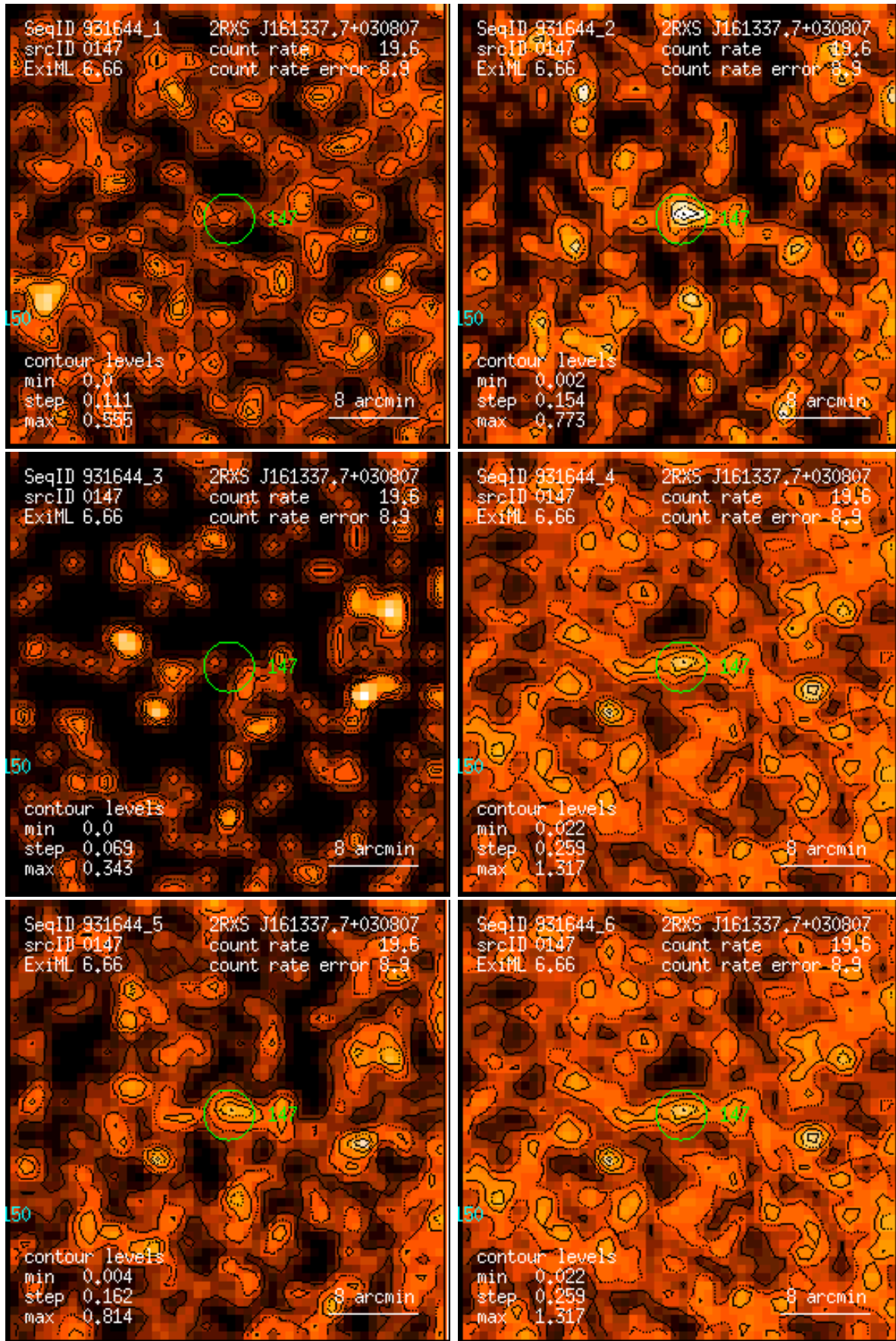
Figure 147: RASS 931644: detection 0147: band rate images, Gaussian filter: (1) PSPC channels 11 – 41, (2) 52 – 90, (3) 91 – 201, (4) 11 – 235, (5) 52 – 201, (6) 11 – 201. Broad band rates in counts/ks. Band rate contour levels in counts/ks/arcmin 2 .
