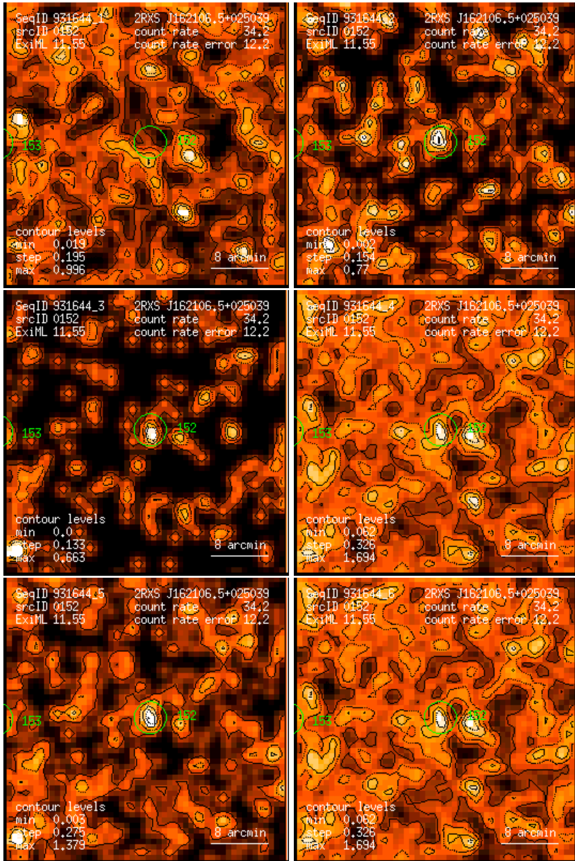
Figure 152: RASS 931644: detection 0152: band rate images, Gaussian filter: (1) PSPC channels 11 – 41, (2) 52 – 90, (3) 91 – 201, (4) 11 – 235, (5) 52 – 201, (6) 11 – 201. Broad band rates in counts/ks. Band rate contour levels in counts/ks/arcmin 2 .
