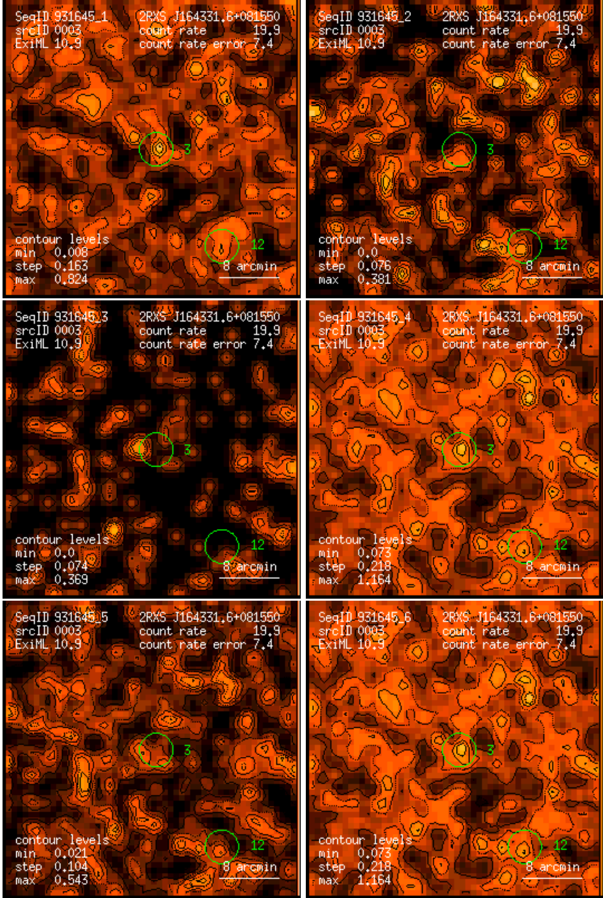
Figure 3: RASS 931645: detection 0003: band rate images, Gaussian filter: (1) PSPC channels 11 – 41, (2) 52 – 90, (3) 91 – 201, (4) 11 – 235, (5) 52 – 201, (6) 11 – 201. Broad band rates in counts/ks. Band rate contour levels in counts/ks/arcmin 2 .
