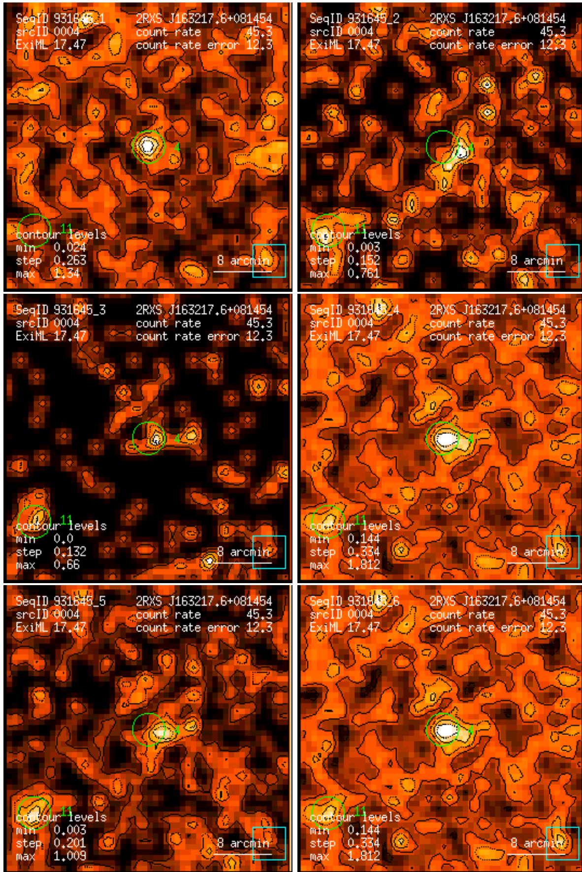
Figure 4: RASS 931645: detection 0004: band rate images, Gaussian filter: (1) PSPC channels 11 – 41, (2) 52 – 90, (3) 91 – 201, (4) 11 – 235, (5) 52 – 201, (6) 11 – 201. Broad band rates in counts/ks. Band rate contour levels in counts/ks/arcmin 2 .
