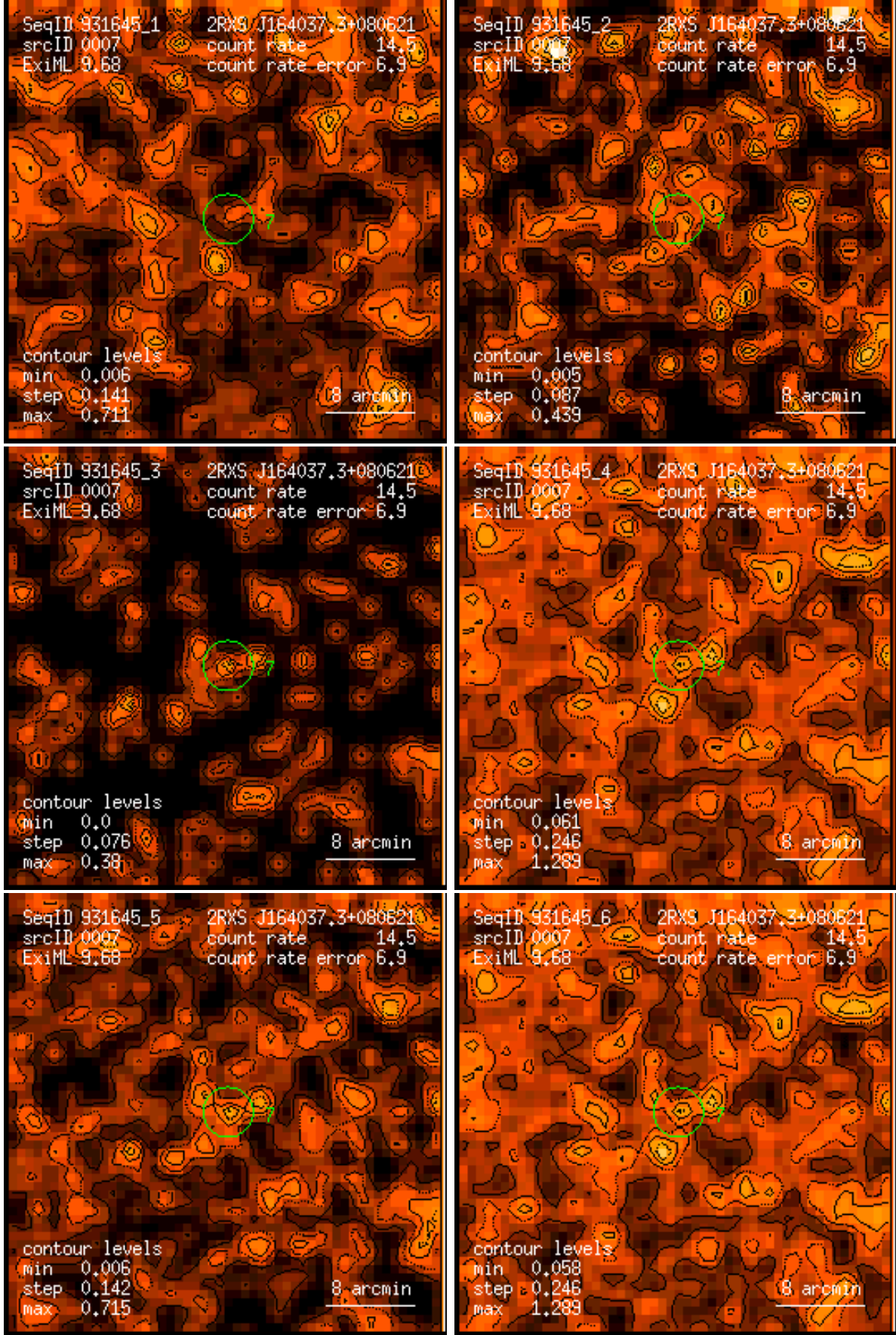
Figure 7: RASS 931645: detection 0007: band rate images, Gaussian filter: (1) PSPC channels 11 – 41, (2) 52 – 90, (3) 91 – 201, (4) 11 – 235, (5) 52 – 201, (6) 11 – 201. Broad band rates in counts/ks. Band rate contour levels in counts/ks/arcmin 2 .
