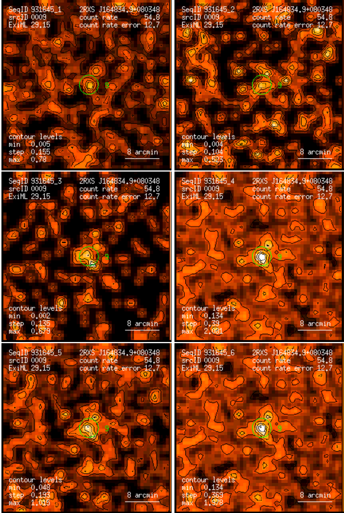
Figure 9: RASS 931645: detection 0009: band rate images, Gaussian filter: (1) PSPC channels 11 – 41, (2) 52 – 90, (3) 91 – 201, (4) 11 – 235, (5) 52 – 201, (6) 11 – 201. Broad band rates in counts/ks. Band rate contour levels in counts/ks/arcmin 2 .
