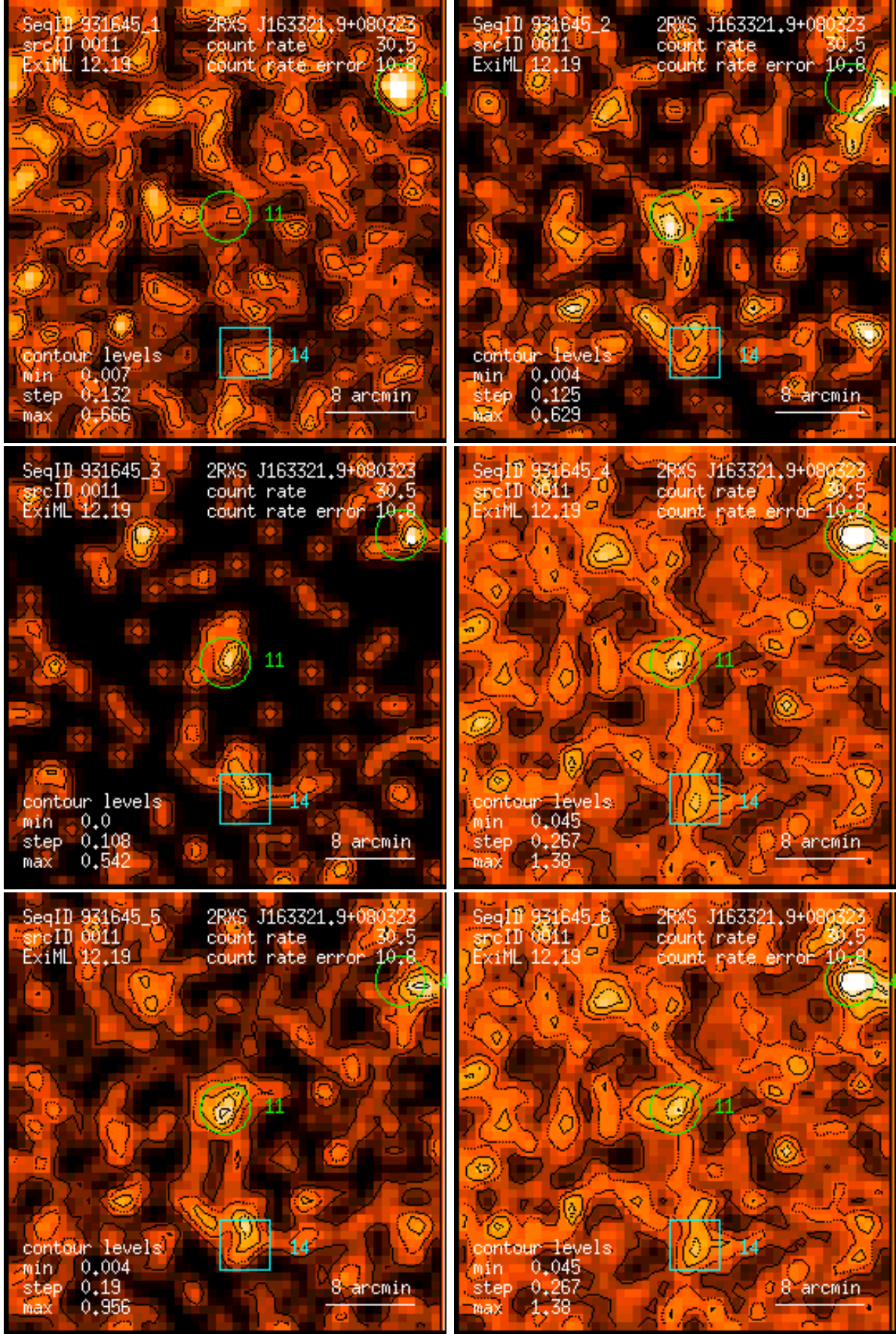
Figure 11: RASS 931645: detection 0011: band rate images, Gaussian filter: (1) PSPC channels 11 – 41, (2) 52 – 90, (3) 91 – 201, (4) 11 – 235, (5) 52 – 201, (6) 11 – 201. Broad band rates in counts/ks. Band rate contour levels in counts/ks/arcmin 2 .
