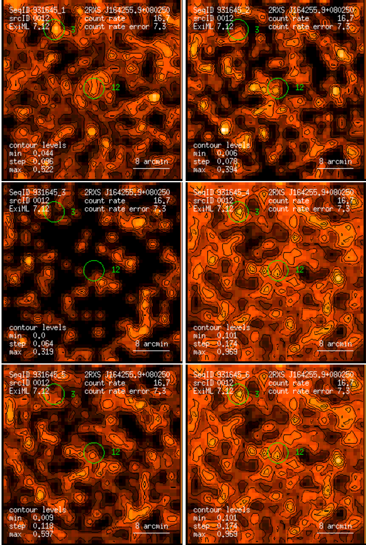
Figure 12: RASS 931645: detection 0012: band rate images, Gaussian filter: (1) PSPC channels 11 – 41, (2) 52 – 90, (3) 91 – 201, (4) 11 – 235, (5) 52 – 201, (6) 11 – 201. Broad band rates in counts/ks. Band rate contour levels in counts/ks/arcmin 2 .
