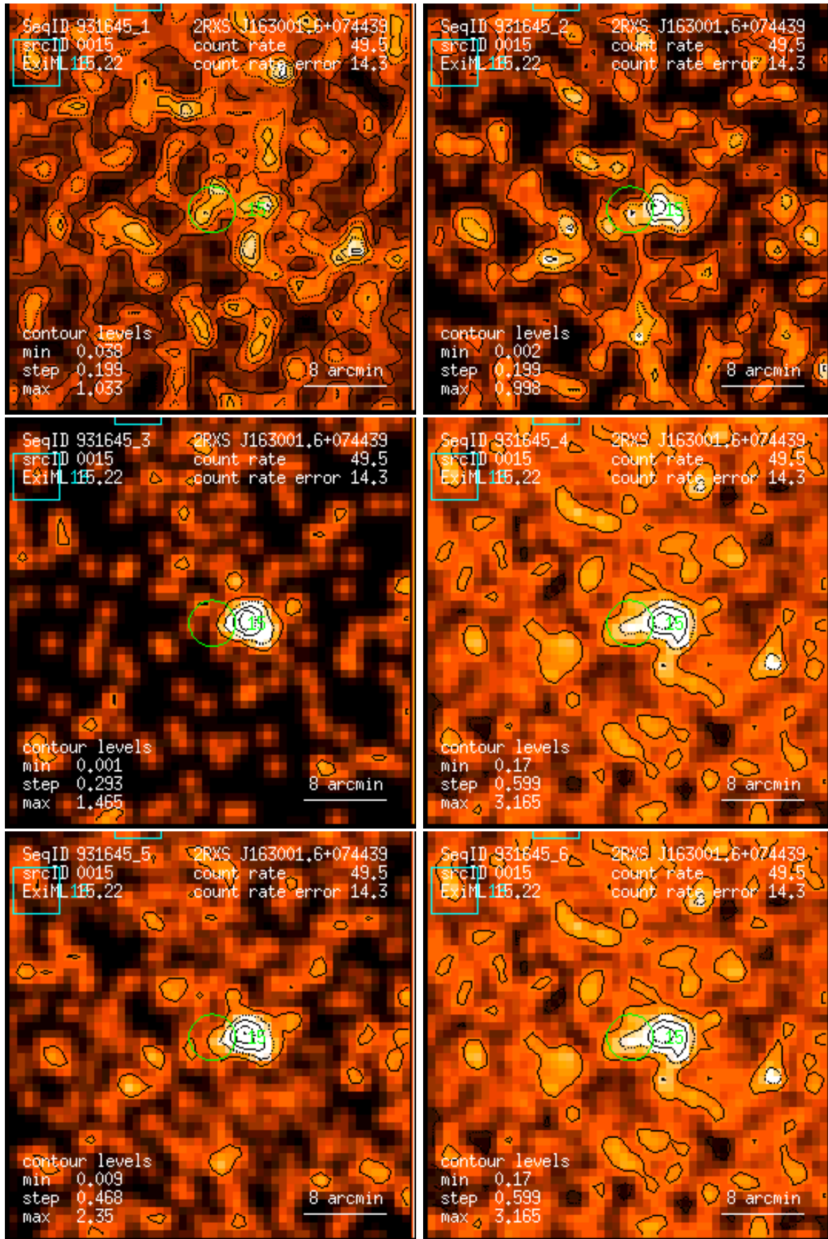
Figure 15: RASS 931645: detection 0015: band rate images, Gaussian filter: (1) PSPC channels 11 – 41, (2) 52 – 90, (3) 91 – 201, (4) 11 – 235, (5) 52 – 201, (6) 11 – 201. Broad band rates in counts/ks. Band rate contour levels in counts/ks/arcmin 2 .
