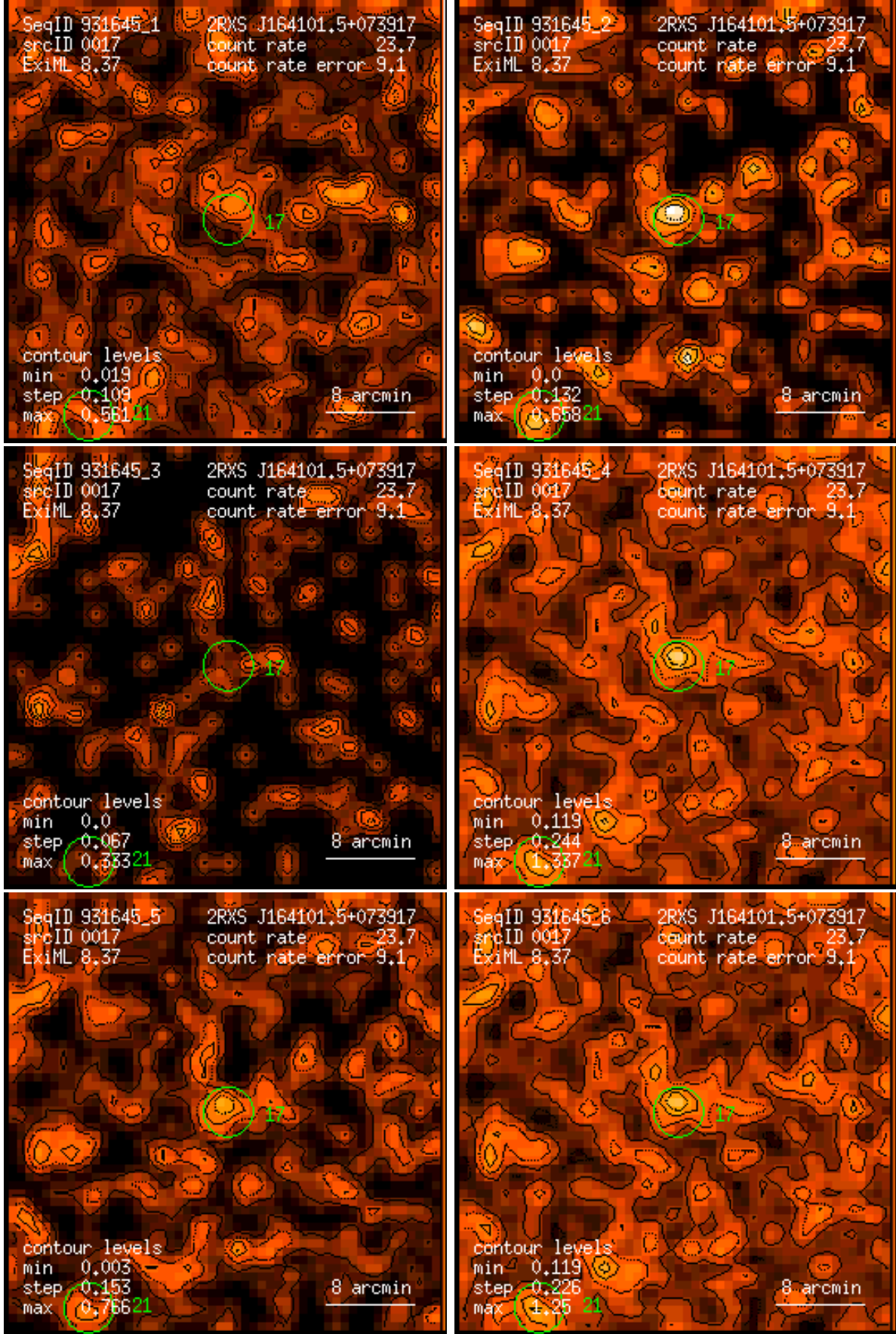
Figure 17: RASS 931645: detection 0017: band rate images, Gaussian filter: (1) PSPC channels 11 – 41, (2) 52 – 90, (3) 91 – 201, (4) 11 – 235, (5) 52 – 201, (6) 11 – 201. Broad band rates in counts/ks. Band rate contour levels in counts/ks/arcmin 2 .
