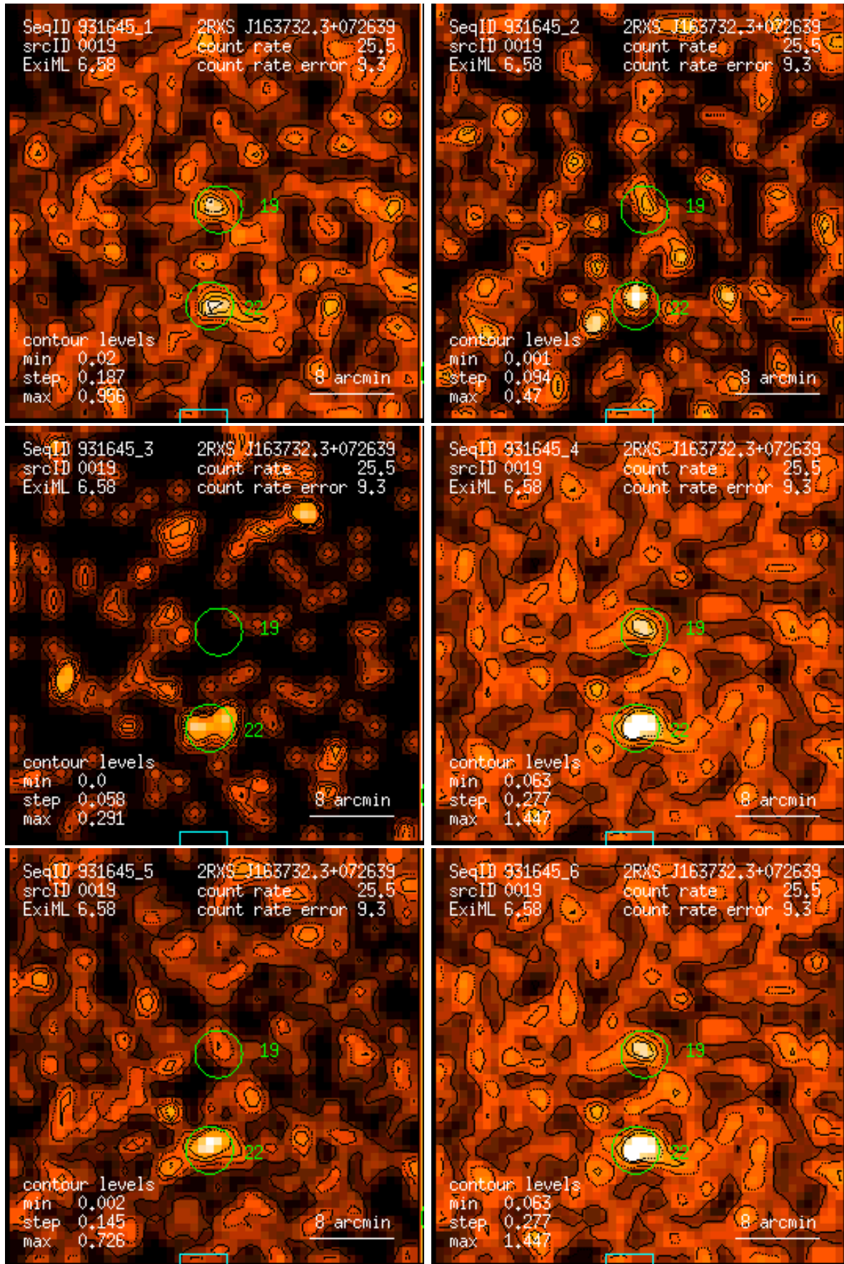
Figure 19: RASS 931645: detection 0019: band rate images, Gaussian filter: (1) PSPC channels 11 – 41, (2) 52 – 90, (3) 91 – 201, (4) 11 – 235, (5) 52 – 201, (6) 11 – 201. Broad band rates in counts/ks. Band rate contour levels in counts/ks/arcmin 2 .
