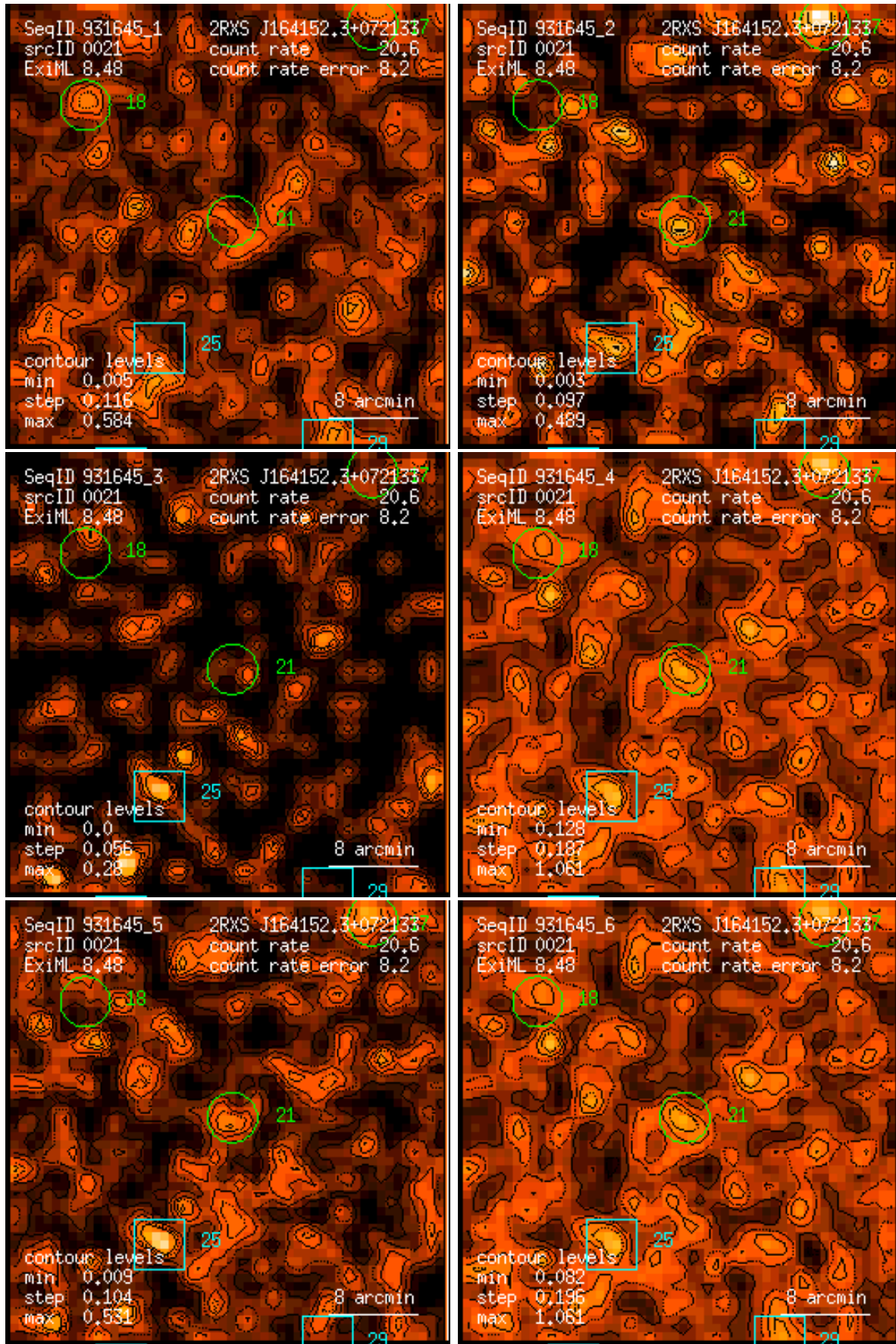
Figure 21: RASS 931645: detection 0021: band rate images, Gaussian filter: (1) PSPC channels 11 – 41, (2) 52 – 90, (3) 91 – 201, (4) 11 – 235, (5) 52 – 201, (6) 11 – 201. Broad band rates in counts/ks. Band rate contour levels in counts/ks/arcmin 2 .
