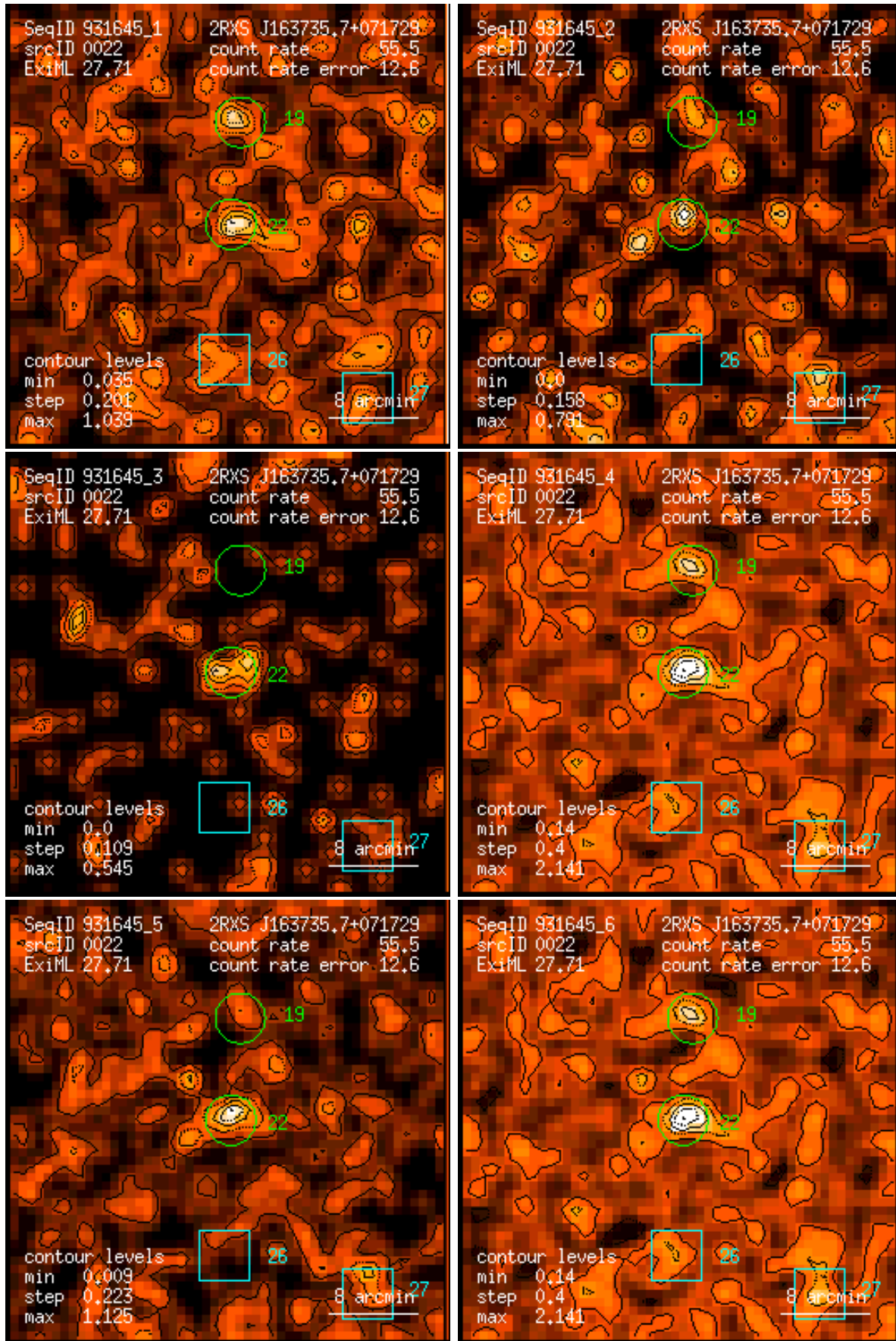
Figure 22: RASS 931645: detection 0022: band rate images, Gaussian filter: (1) PSPC channels 11 – 41, (2) 52 – 90, (3) 91 – 201, (4) 11 – 235, (5) 52 – 201, (6) 11 – 201. Broad band rates in counts/ks. Band rate contour levels in counts/ks/arcmin 2 .
