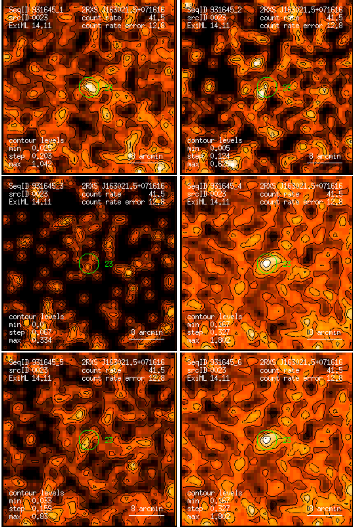
Figure 23: RASS 931645: detection 0023: band rate images, Gaussian filter: (1) PSPC channels 11 – 41, (2) 52 – 90, (3) 91 – 201, (4) 11 – 235, (5) 52 – 201, (6) 11 – 201. Broad band rates in counts/ks. Band rate contour levels in counts/ks/arcmin 2 .
