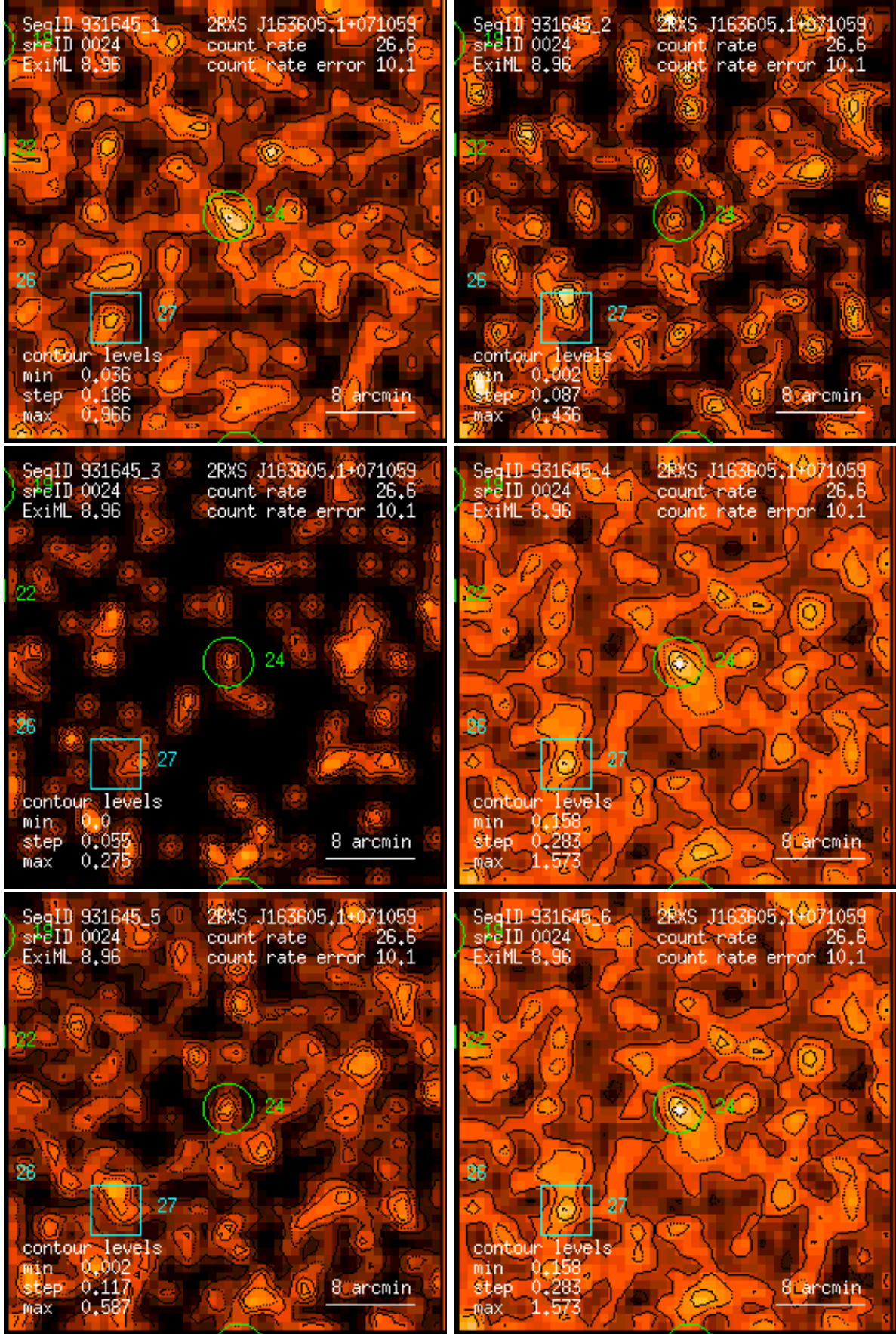
Figure 24: RASS 931645: detection 0024: band rate images, Gaussian filter: (1) PSPC channels 11 – 41, (2) 52 – 90, (3) 91 – 201, (4) 11 – 235, (5) 52 – 201, (6) 11 – 201. Broad band rates in counts/ks. Band rate contour levels in counts/ks/arcmin 2 .
