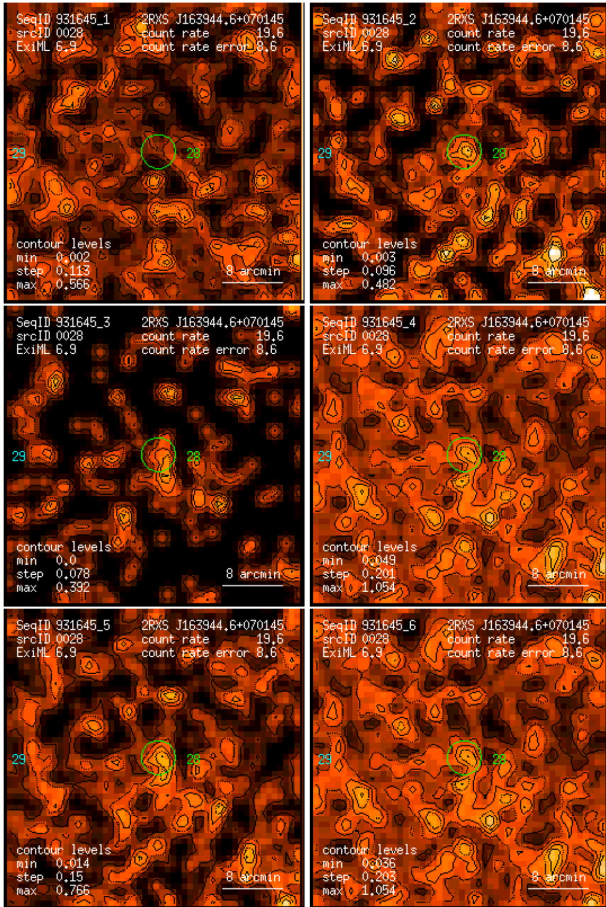
Figure 28: RASS 931645: detection 0028: band rate images, Gaussian filter: (1) PSPC channels 11 – 41, (2) 52 – 90, (3) 91 – 201, (4) 11 – 235, (5) 52 – 201, (6) 11 – 201. Broad band rates in counts/ks. Band rate contour levels in counts/ks/arcmin 2 .
