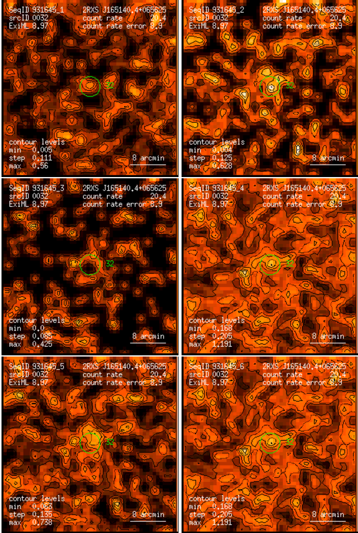
Figure 32: RASS 931645: detection 0032: band rate images, Gaussian filter: (1) PSPC channels 11 – 41, (2) 52 – 90, (3) 91 – 201, (4) 11 – 235, (5) 52 – 201, (6) 11 – 201. Broad band rates in counts/ks. Band rate contour levels in counts/ks/arcmin 2 .
