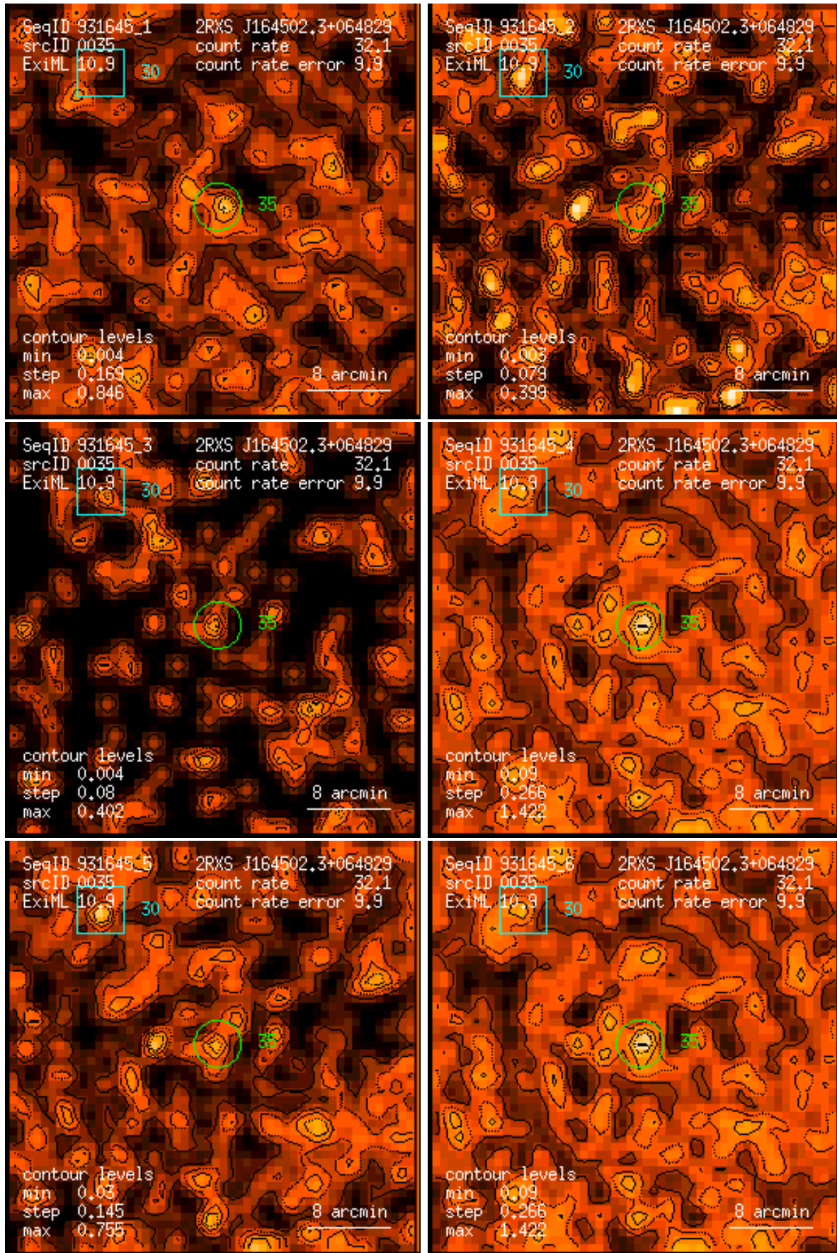
Figure 35: RASS 931645: detection 0035: band rate images, Gaussian filter: (1) PSPC channels 11 – 41, (2) 52 – 90, (3) 91 – 201, (4) 11 – 235, (5) 52 – 201, (6) 11 – 201. Broad band rates in counts/ks. Band rate contour levels in counts/ks/arcmin 2 .
