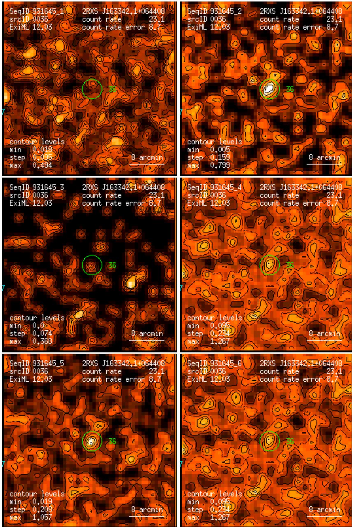
Figure 36: RASS 931645: detection 0036: band rate images, Gaussian filter: (1) PSPC channels 11 – 41, (2) 52 – 90, (3) 91 – 201, (4) 11 – 235, (5) 52 – 201, (6) 11 – 201. Broad band rates in counts/ks. Band rate contour levels in counts/ks/arcmin 2 .
